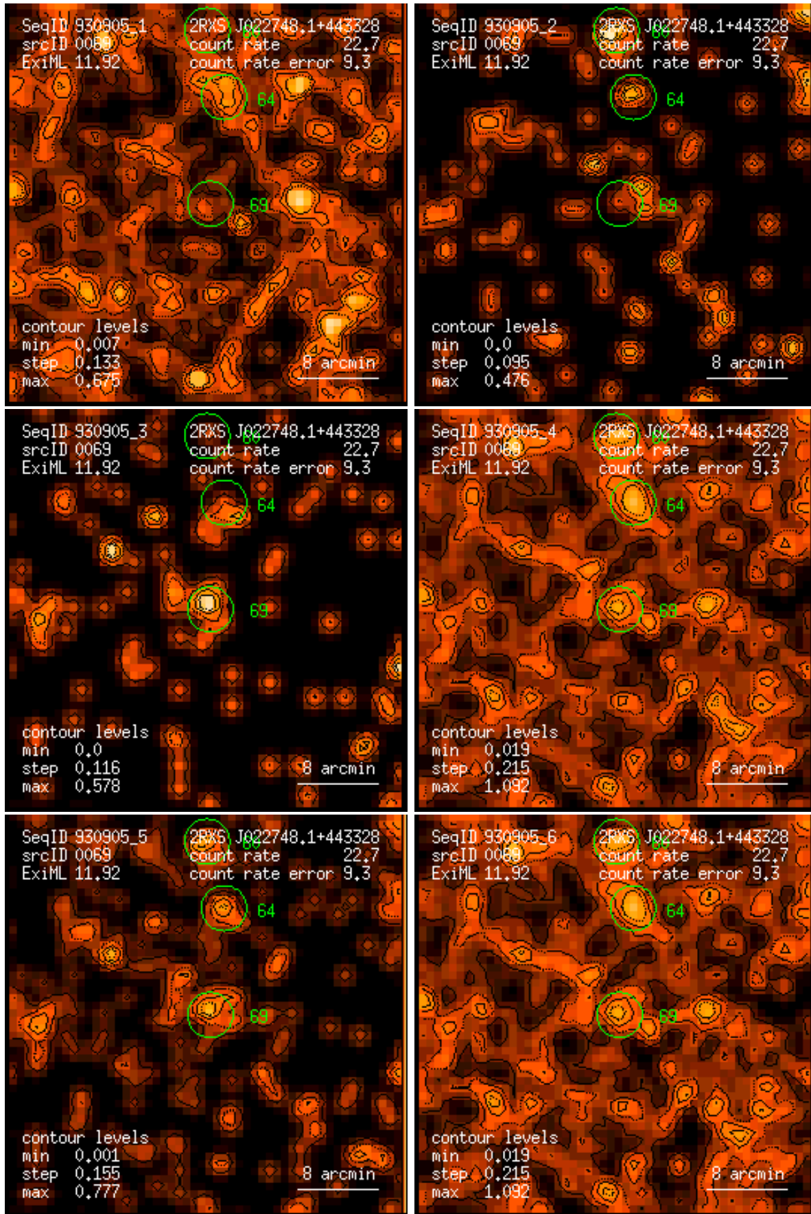
Figure 69: RASS 930905: detection 0069: band rate images, Gaussian filter: (1) PSPC channels 11 – 41, (2) 52 – 90, (3) 91 – 201, (4) 11 – 235, (5) 52 – 201, (6) 11 – 201. Broad band rates in counts/ks. Band rate contour levels in counts/ks/arcmin 2 .
