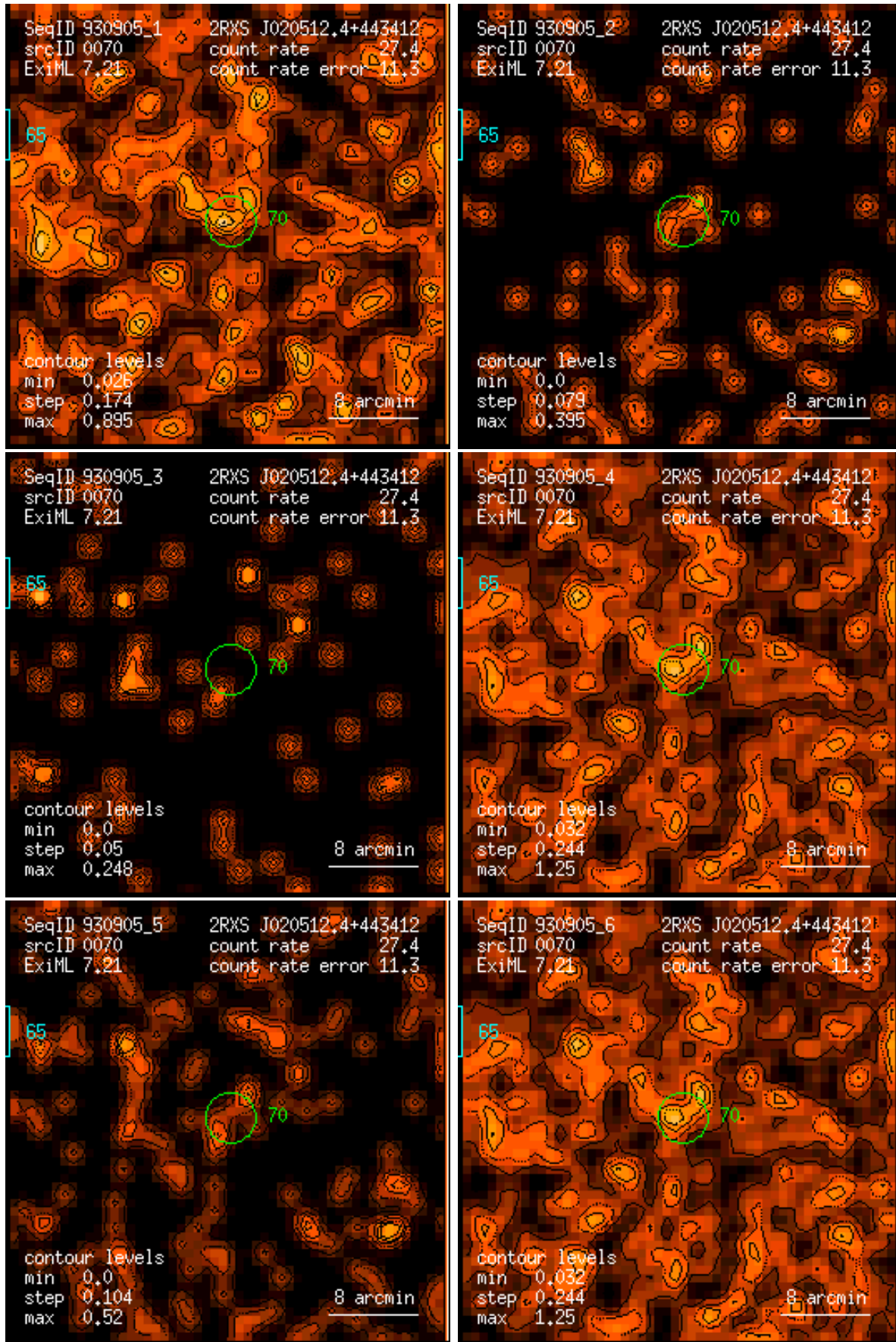
Figure 70: RASS 930905: detection 0070: band rate images, Gaussian filter: (1) PSPC channels 11 – 41, (2) 52 – 90, (3) 91 – 201, (4) 11 – 235, (5) 52 – 201, (6) 11 – 201. Broad band rates in counts/ks. Band rate contour levels in counts/ks/arcmin 2 .
