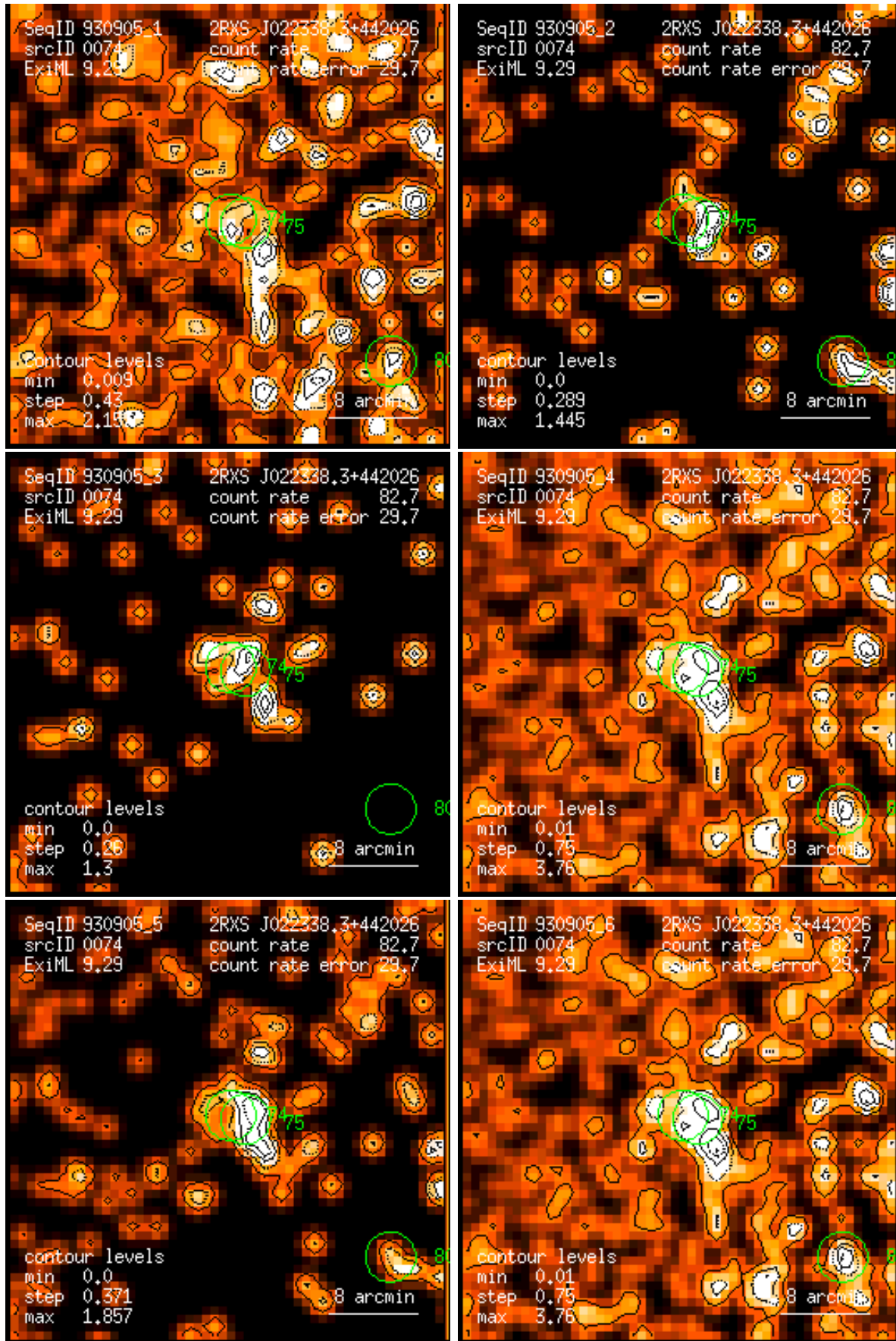
Figure 74: RASS 930905: detection 0074: band rate images, Gaussian filter: (1) PSPC channels 11 – 41, (2) 52 – 90, (3) 91 – 201, (4) 11 – 235, (5) 52 – 201, (6) 11 – 201. Broad band rates in counts/ks. Band rate contour levels in counts/ks/arcmin 2 .
