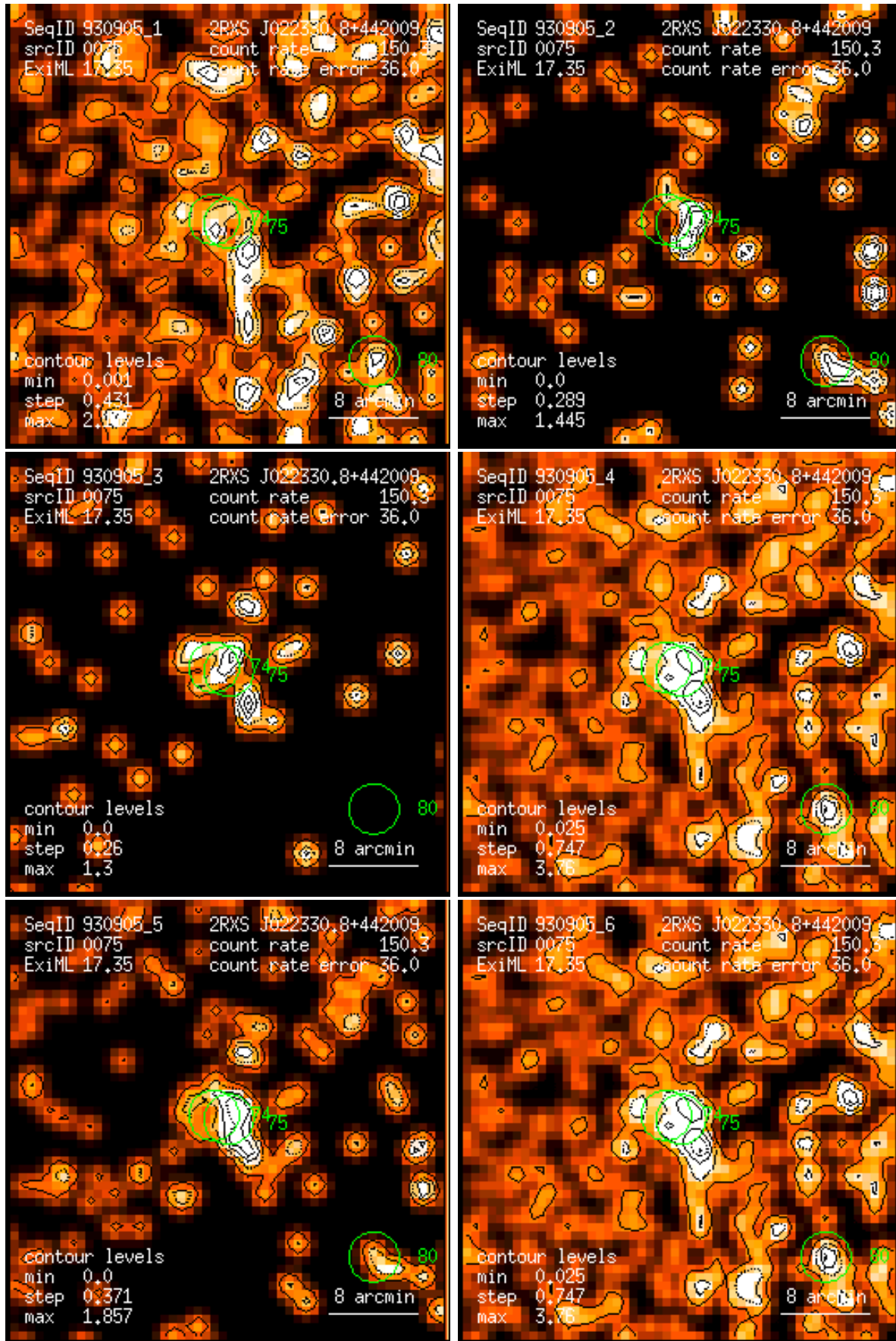
Figure 75: RASS 930905: detection 0075: band rate images, Gaussian filter: (1) PSPC channels 11 – 41, (2) 52 – 90, (3) 91 – 201, (4) 11 – 235, (5) 52 – 201, (6) 11 – 201. Broad band rates in counts/ks. Band rate contour levels in counts/ks/arcmin 2 .
