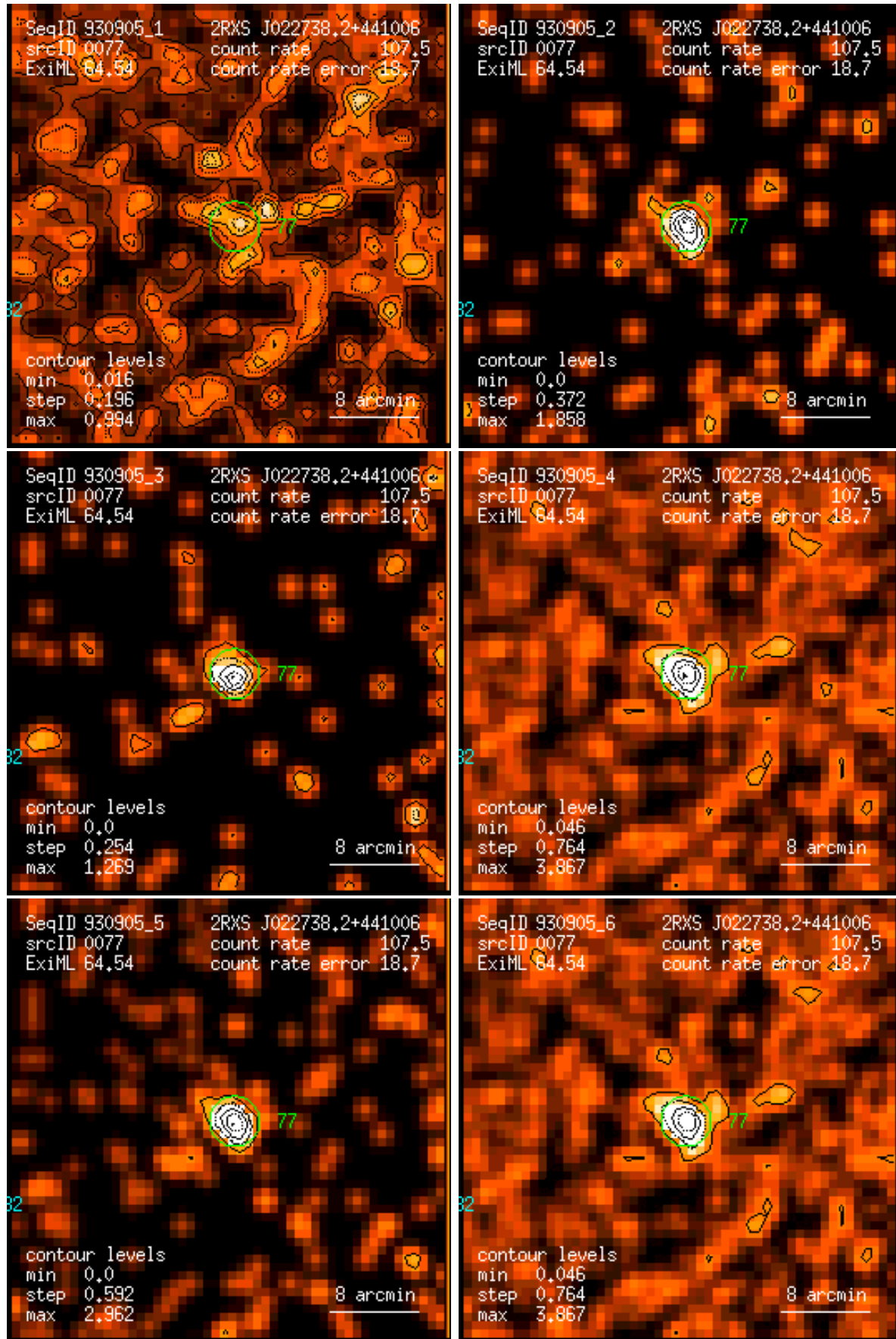
Figure 77: RASS 930905: detection 0077: band rate images, Gaussian filter: (1) PSPC channels 11 – 41, (2) 52 – 90, (3) 91 – 201, (4) 11 – 235, (5) 52 – 201, (6) 11 – 201. Broad band rates in counts/ks. Band rate contour levels in counts/ks/arcmin 2 .
