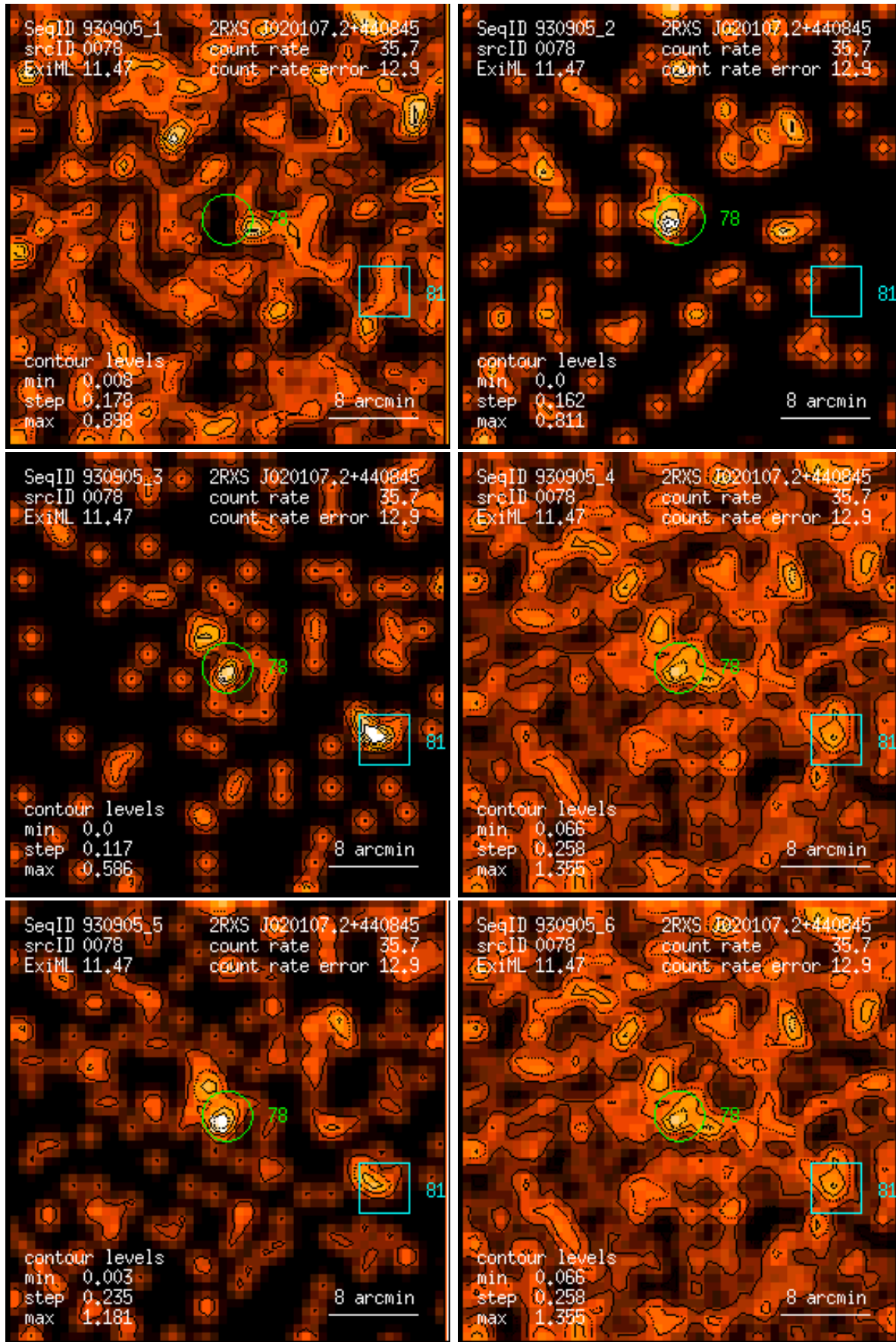
Figure 78: RASS 930905: detection 0078: band rate images, Gaussian filter: (1) PSPC channels 11 – 41, (2) 52 – 90, (3) 91 – 201, (4) 11 – 235, (5) 52 – 201, (6) 11 – 201. Broad band rates in counts/ks. Band rate contour levels in counts/ks/arcmin 2 .
