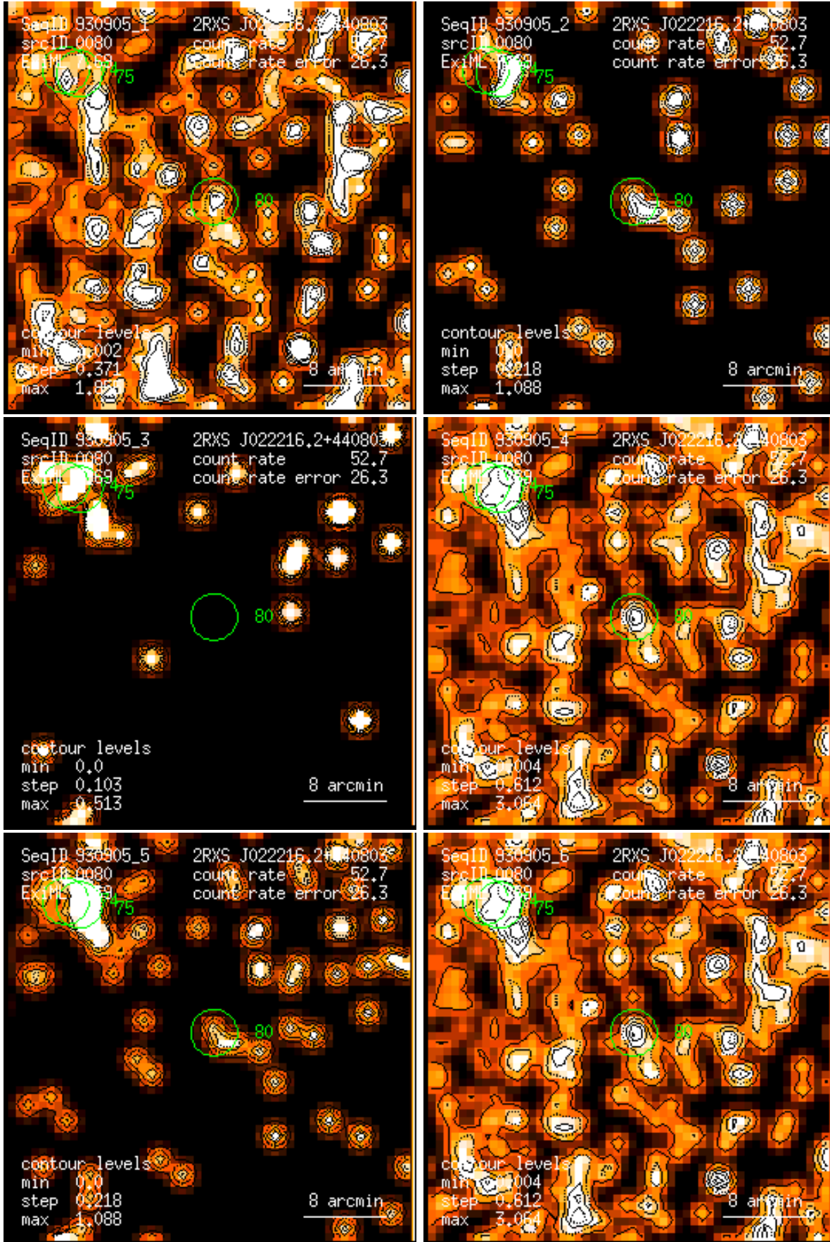
Figure 80: RASS 930905: detection 0080: band rate images, Gaussian filter: (1) PSPC channels 11 – 41, (2) 52 – 90, (3) 91 – 201, (4) 11 – 235, (5) 52 – 201, (6) 11 – 201. Broad band rates in counts/ks. Band rate contour levels in counts/ks/arcmin 2 .
