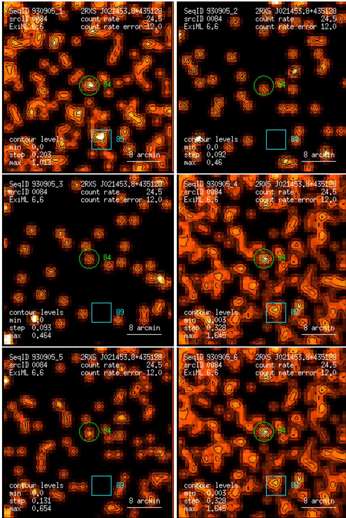
Figure 84: RASS 930905: detection 0084: band rate images, Gaussian filter: (1) PSPC channels 11 – 41, (2) 52 – 90, (3) 91 – 201, (4) 11 – 235, (5) 52 – 201, (6) 11 – 201. Broad band rates in counts/ks. Band rate contour levels in counts/ks/arcmin 2 .
