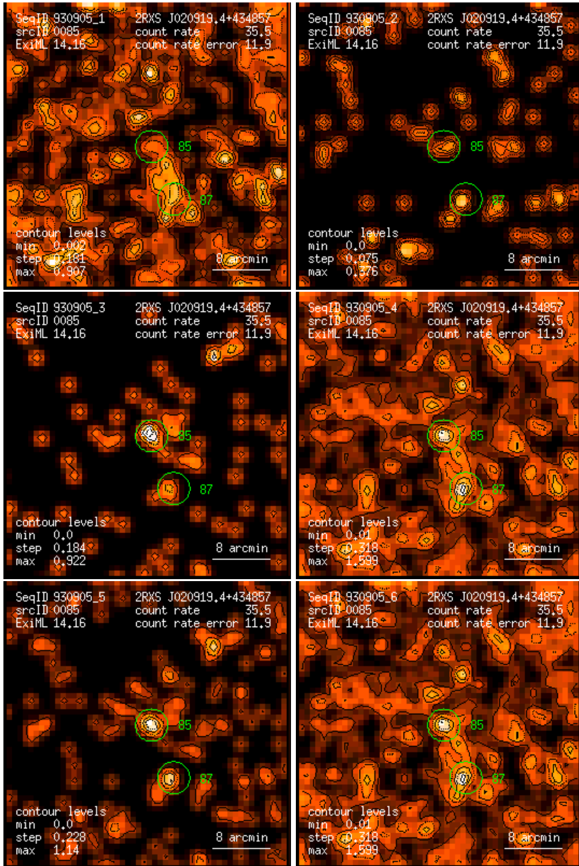
Figure 85: RASS 930905: detection 0085: band rate images, Gaussian filter: (1) PSPC channels 11 – 41, (2) 52 – 90, (3) 91 – 201, (4) 11 – 235, (5) 52 – 201, (6) 11 – 201. Broad band rates in counts/ks. Band rate contour levels in counts/ks/arcmin 2 .
