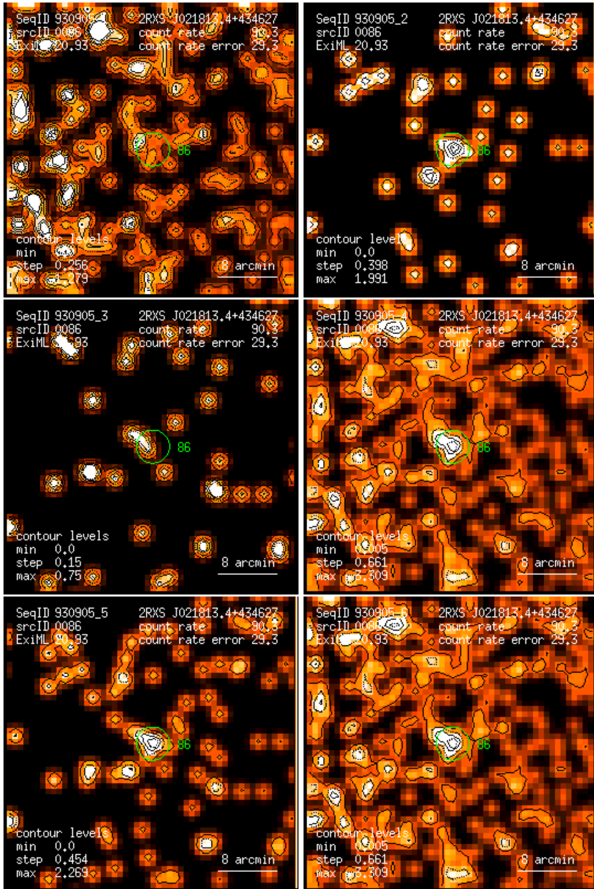
Figure 86: RASS 930905: detection 0086: band rate images, Gaussian filter: (1) PSPC channels 11 – 41, (2) 52 – 90, (3) 91 – 201, (4) 11 – 235, (5) 52 – 201, (6) 11 – 201. Broad band rates in counts/ks. Band rate contour levels in counts/ks/arcmin 2 .
