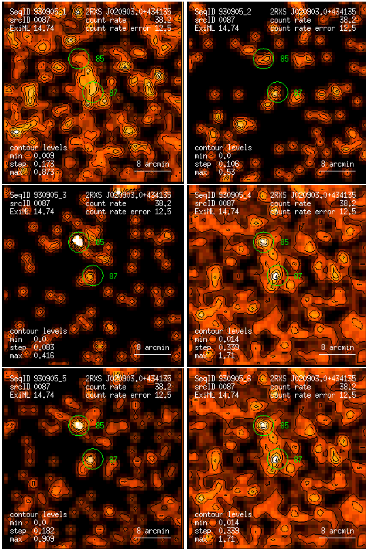
Figure 87: RASS 930905: detection 0087: band rate images, Gaussian filter: (1) PSPC channels 11 – 41, (2) 52 – 90, (3) 91 – 201, (4) 11 – 235, (5) 52 – 201, (6) 11 – 201. Broad band rates in counts/ks. Band rate contour levels in counts/ks/arcmin 2 .
