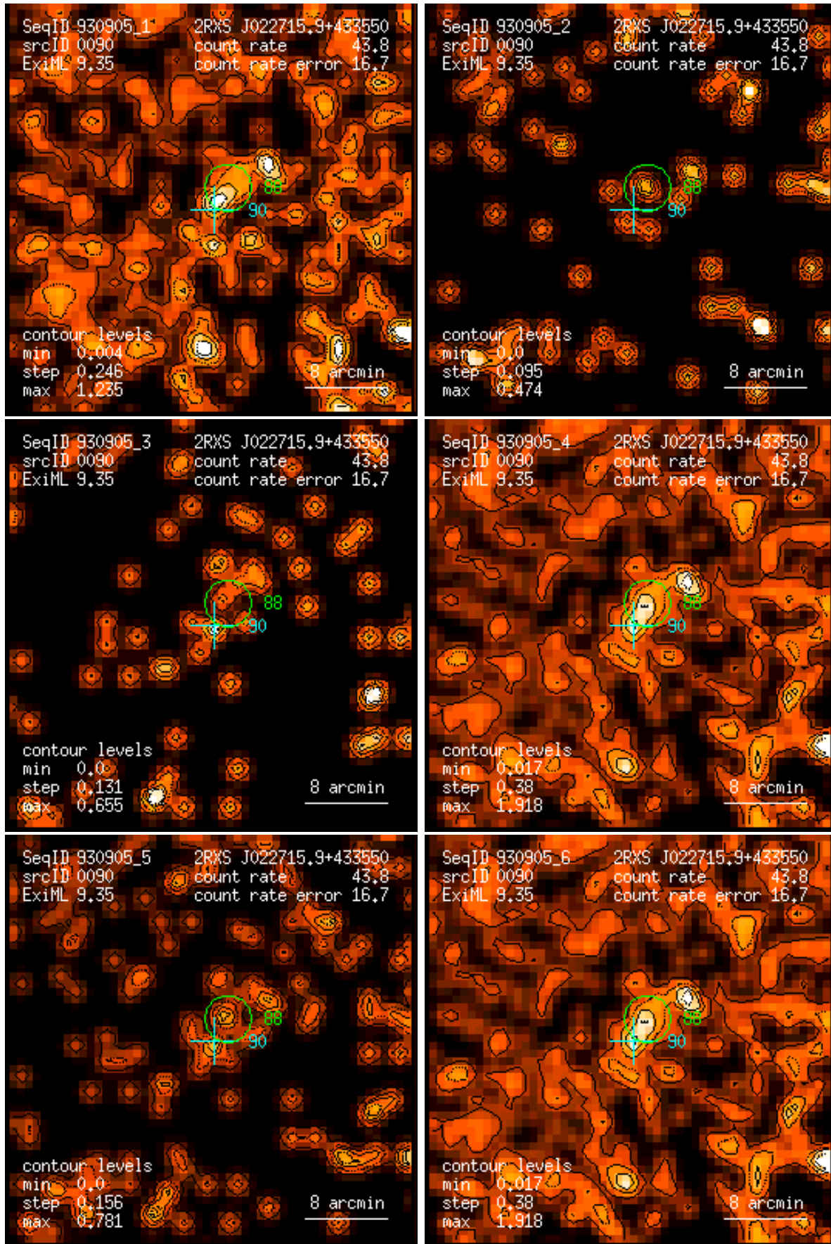
Figure 90: RASS 930905: detection 0090: band rate images, Gaussian filter: (1) PSPC channels 11 – 41, (2) 52 – 90, (3) 91 – 201, (4) 11 – 235, (5) 52 – 201, (6) 11 – 201. Broad band rates in counts/ks. Band rate contour levels in counts/ks/arcmin 2 .
