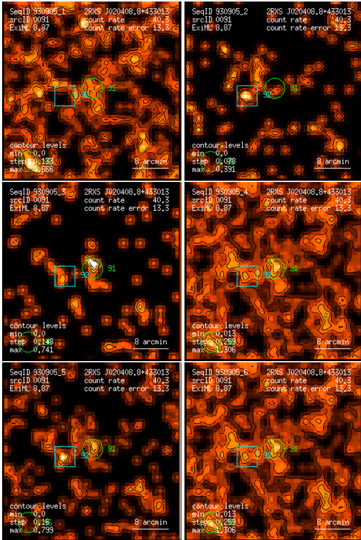
Figure 91: RASS 930905: detection 0091: band rate images, Gaussian filter: (1) PSPC channels 11 – 41, (2) 52 – 90, (3) 91 – 201, (4) 11 – 235, (5) 52 – 201, (6) 11 – 201. Broad band rates in counts/ks. Band rate contour levels in counts/ks/arcmin 2 .
