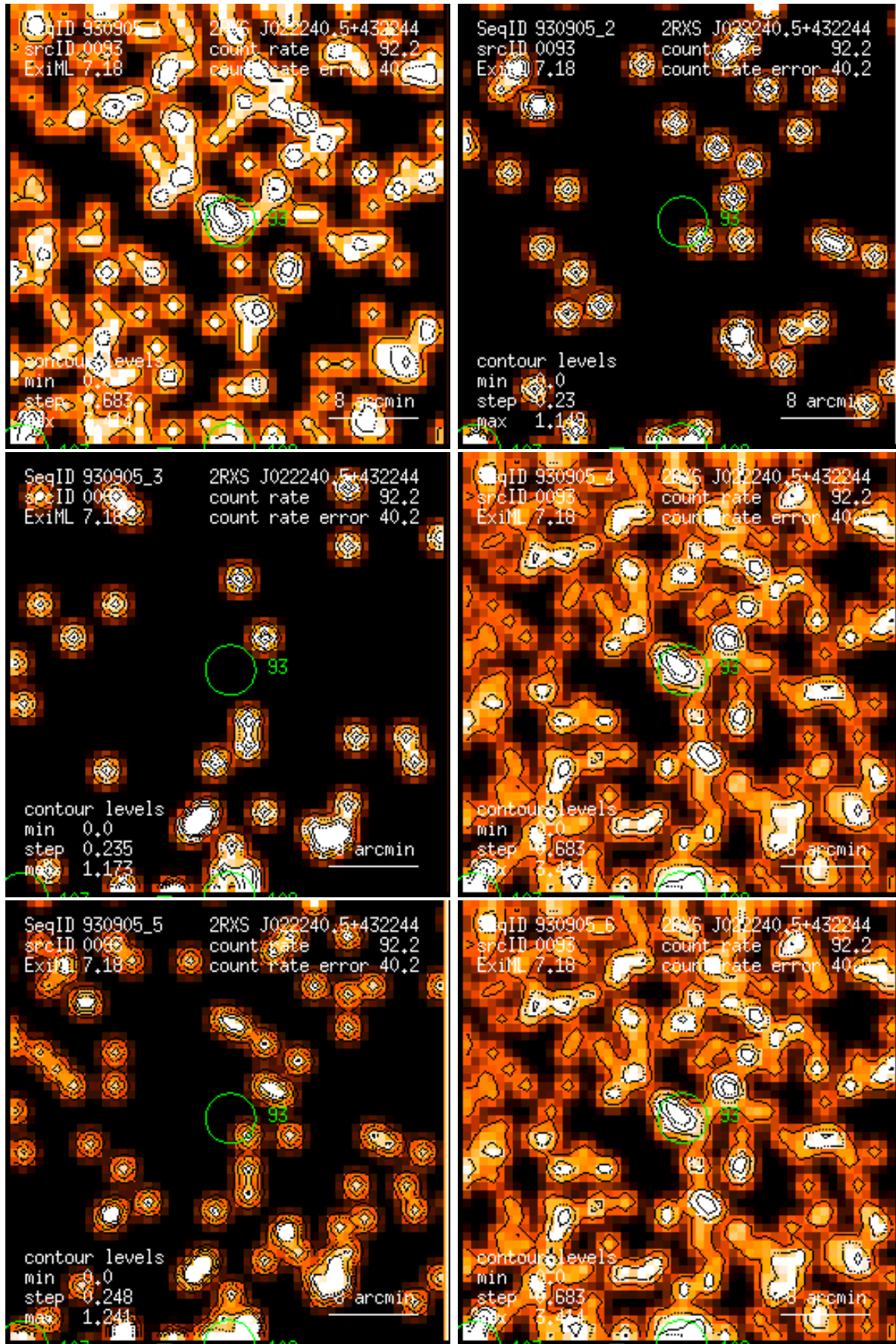
Figure 93: RASS 930905: detection 0093: band rate images, Gaussian filter: (1) PSPC channels 11 – 41, (2) 52 – 90, (3) 91 – 201, (4) 11 – 235, (5) 52 – 201, (6) 11 – 201. Broad band rates in counts/ks. Band rate contour levels in counts/ks/arcmin 2 .
