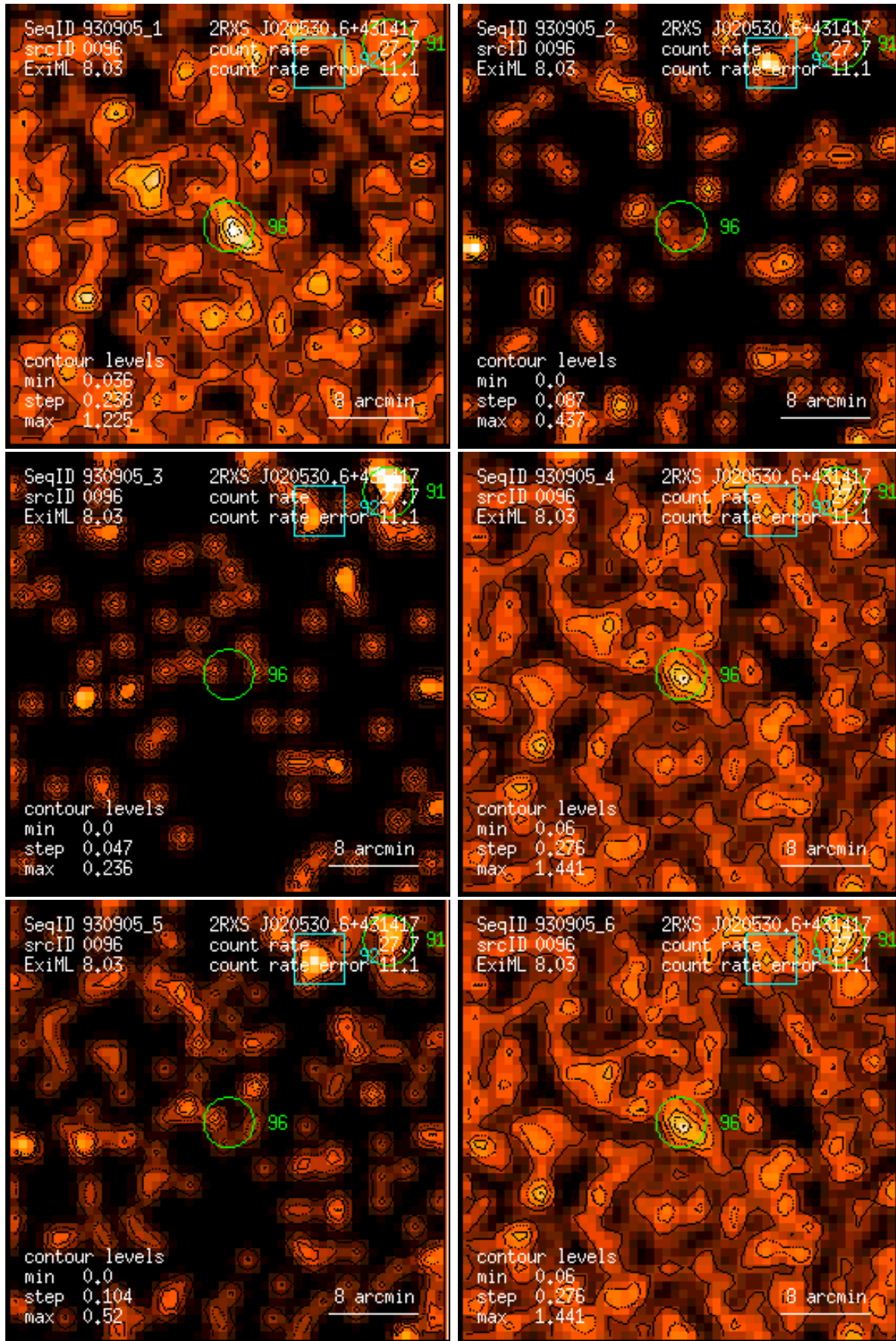
Figure 96: RASS 930905: detection 0096: band rate images, Gaussian filter: (1) PSPC channels 11 – 41, (2) 52 – 90, (3) 91 – 201, (4) 11 – 235, (5) 52 – 201, (6) 11 – 201. Broad band rates in counts/ks. Band rate contour levels in counts/ks/arcmin 2 .
