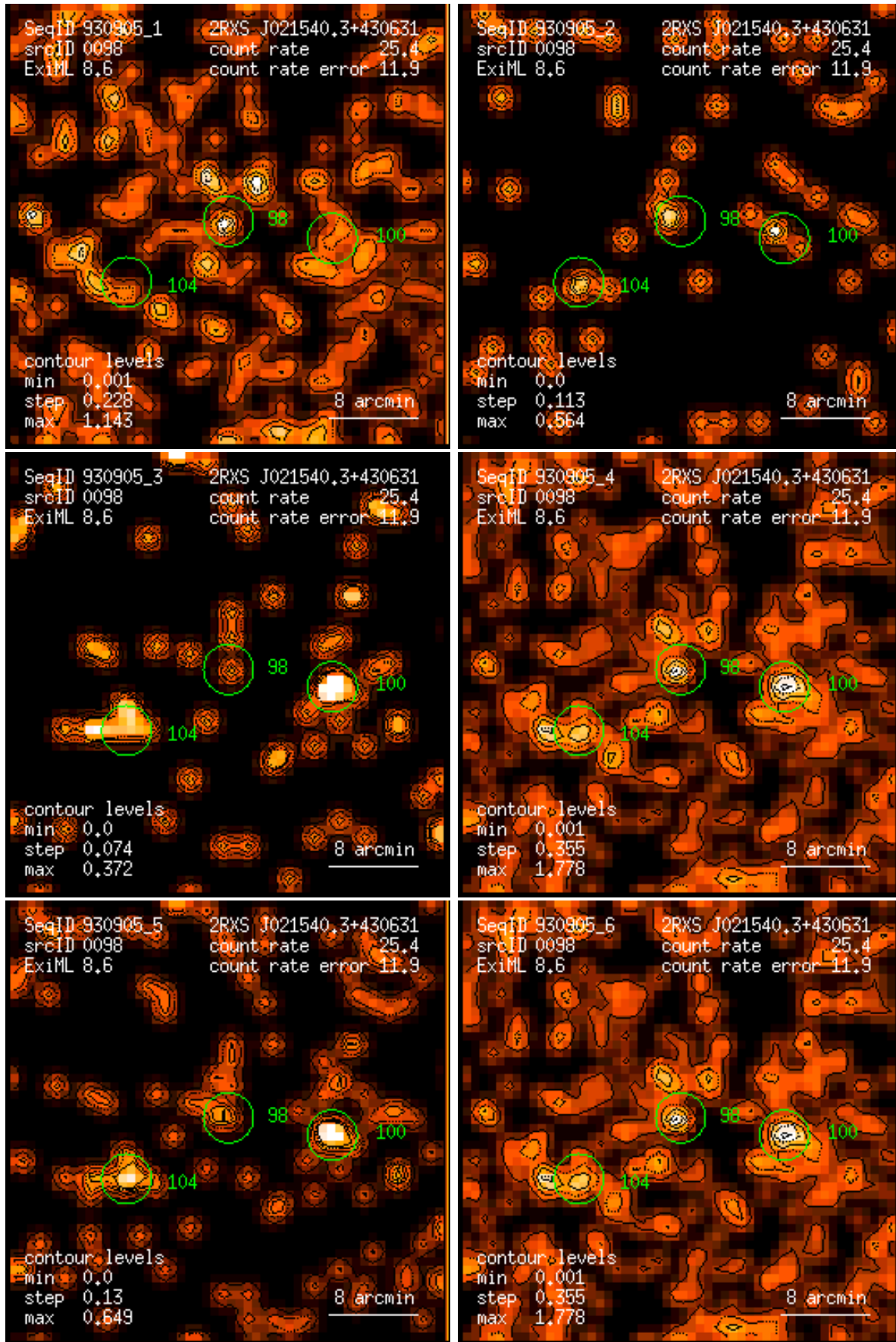
Figure 98: RASS 930905: detection 0098: band rate images, Gaussian filter: (1) PSPC channels 11 – 41, (2) 52 – 90, (3) 91 – 201, (4) 11 – 235, (5) 52 – 201, (6) 11 – 201. Broad band rates in counts/ks. Band rate contour levels in counts/ks/arcmin 2 .
