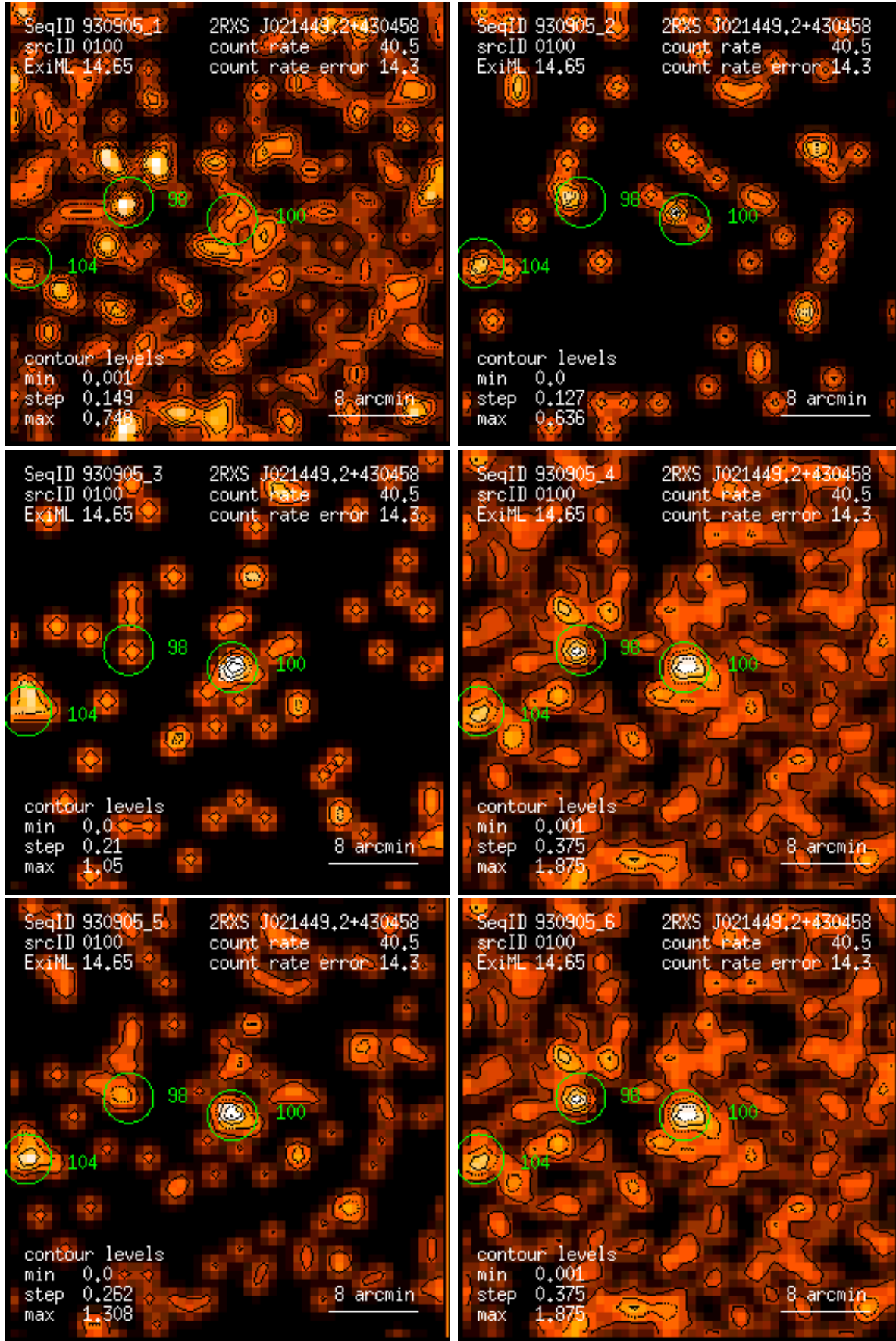
Figure 100: RASS 930905: detection 0100: band rate images, Gaussian filter: (1) PSPC channels 11 – 41, (2) 52 – 90, (3) 91 – 201, (4) 11 – 235, (5) 52 – 201, (6) 11 – 201. Broad band rates in counts/ks. Band rate contour levels in counts/ks/arcmin 2 .
