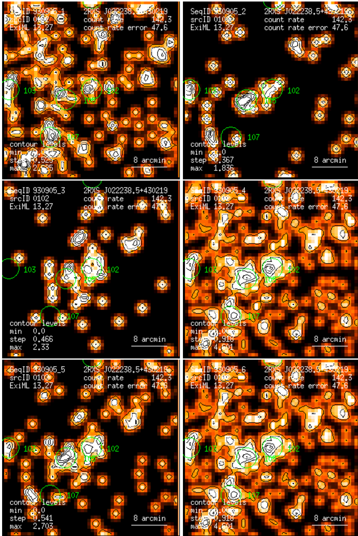
Figure 102: RASS 930905: detection 0102: band rate images, Gaussian filter: (1) PSPC channels 11 – 41, (2) 52 – 90, (3) 91 – 201, (4) 11 – 235, (5) 52 – 201, (6) 11 – 201. Broad band rates in counts/ks. Band rate contour levels in counts/ks/arcmin 2 .
