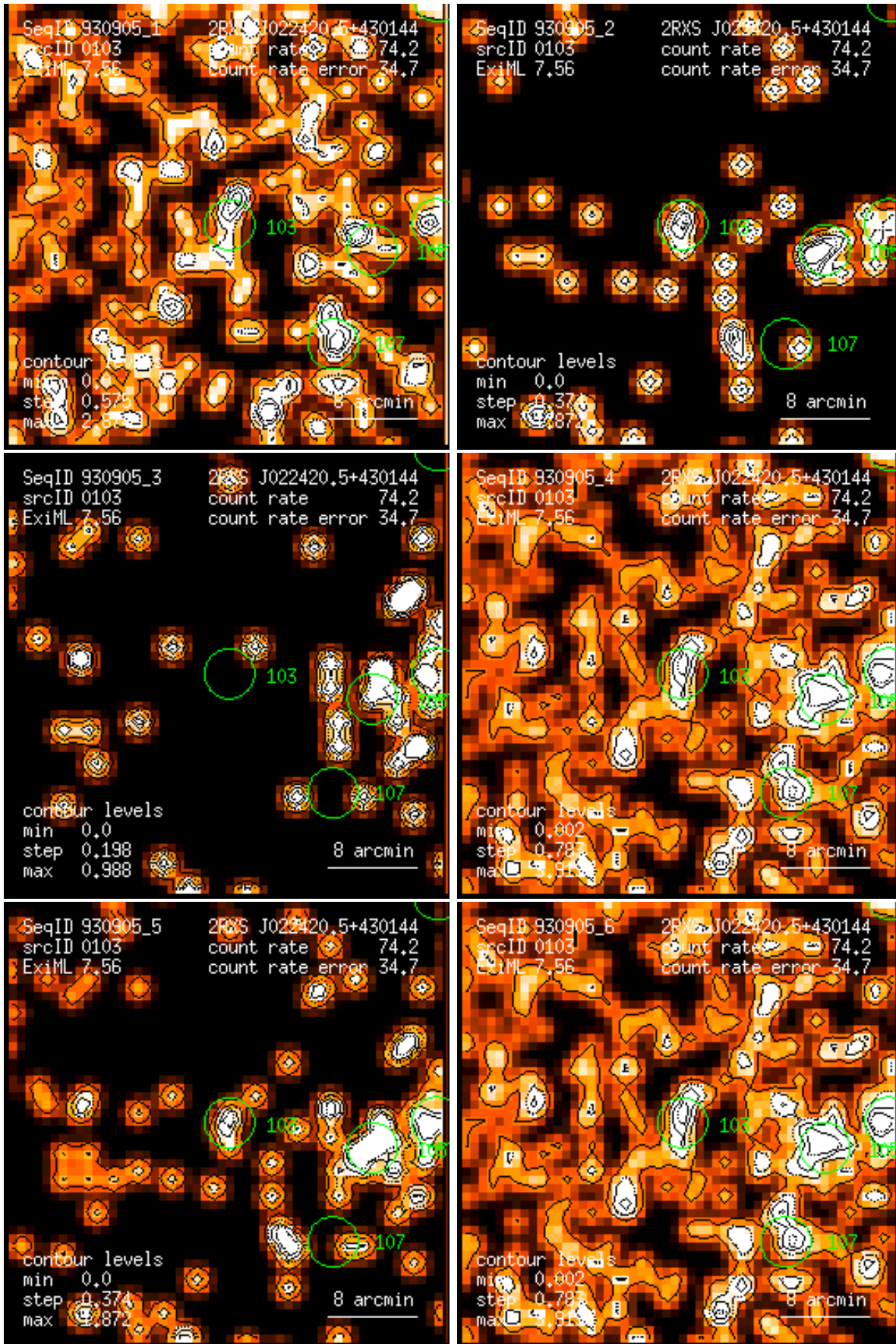
Figure 103: RASS 930905: detection 0103: band rate images, Gaussian filter: (1) PSPC channels 11 – 41, (2) 52 – 90, (3) 91 – 201, (4) 11 – 235, (5) 52 – 201, (6) 11 – 201. Broad band rates in counts/ks. Band rate contour levels in counts/ks/arcmin 2 .
