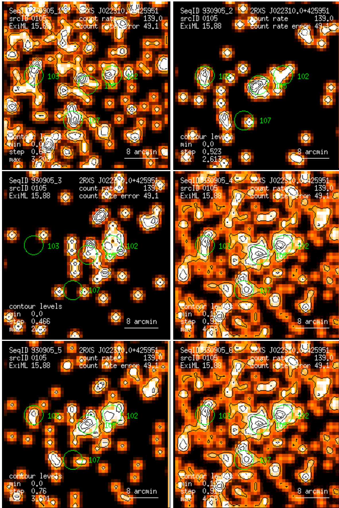
Figure 105: RASS 930905: detection 0105: band rate images, Gaussian filter: (1) PSPC channels 11 – 41, (2) 52 – 90, (3) 91 – 201, (4) 11 – 235, (5) 52 – 201, (6) 11 – 201. Broad band rates in counts/ks. Band rate contour levels in counts/ks/arcmin 2 .
