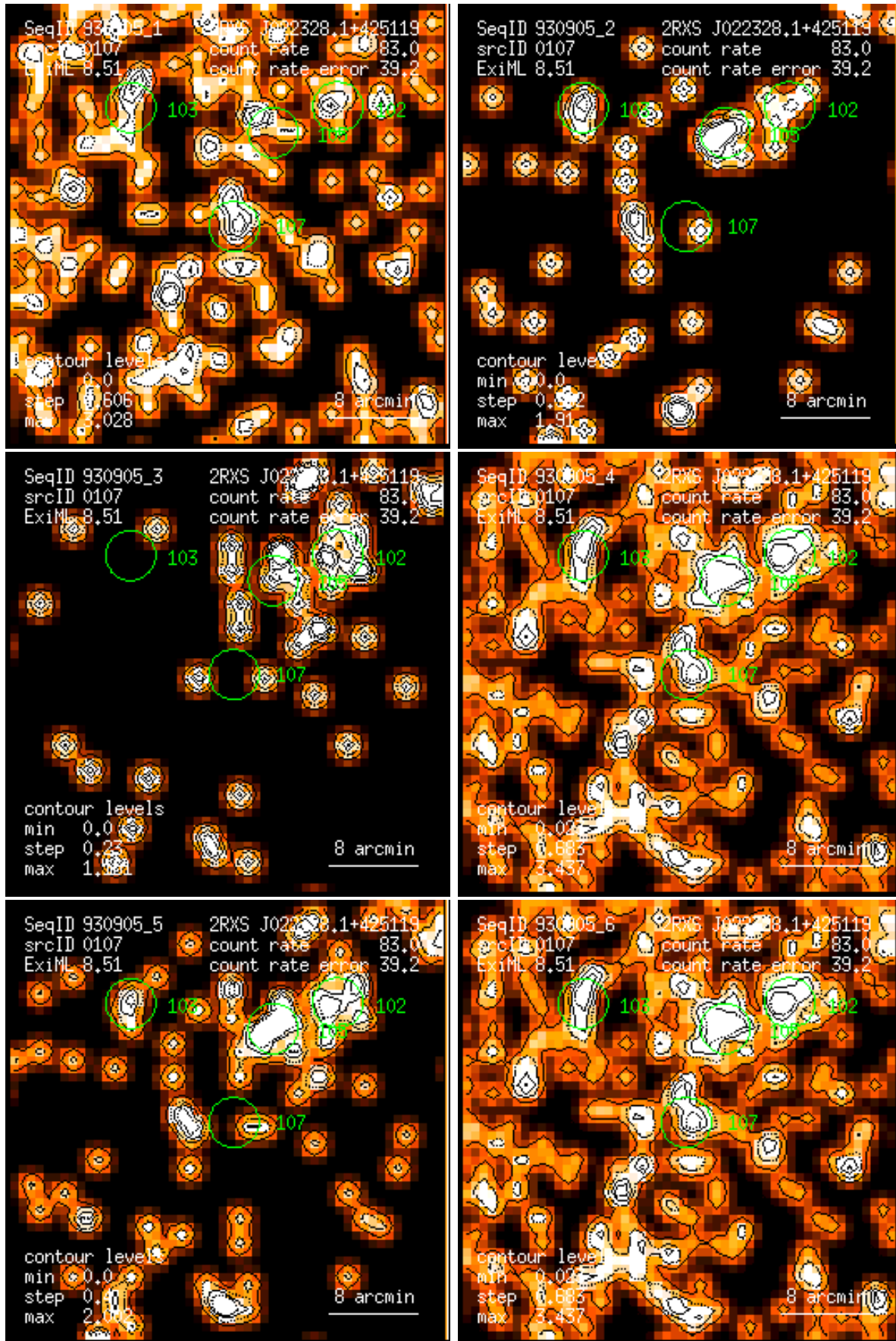
Figure 107: RASS 930905: detection 0107: band rate images, Gaussian filter: (1) PSPC channels 11 – 41, (2) 52 – 90, (3) 91 – 201, (4) 11 – 235, (5) 52 – 201, (6) 11 – 201. Broad band rates in counts/ks. Band rate contour levels in counts/ks/arcmin 2 .
