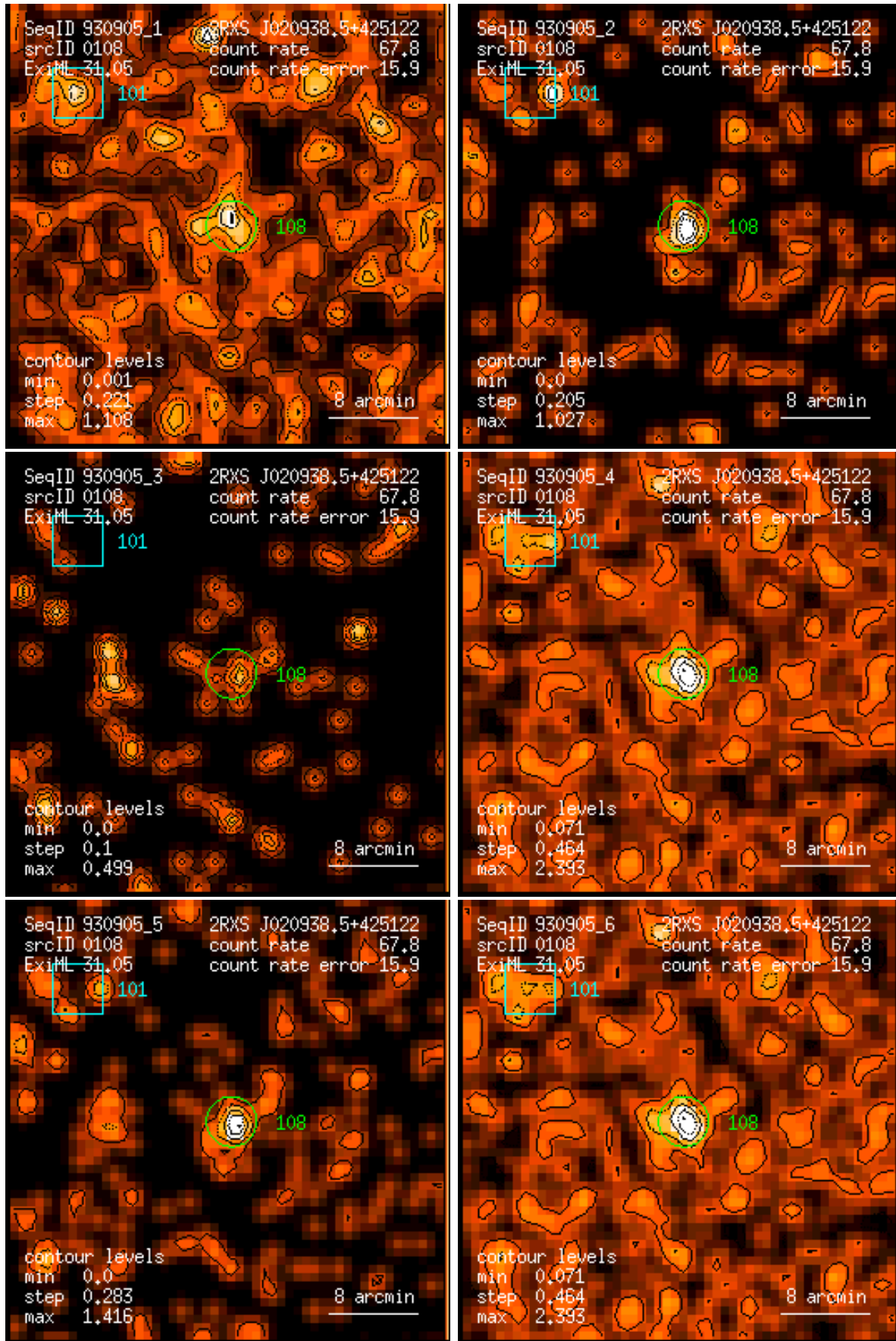
Figure 108: RASS 930905: detection 0108: band rate images, Gaussian filter: (1) PSPC channels 11 – 41, (2) 52 – 90, (3) 91 – 201, (4) 11 – 235, (5) 52 – 201, (6) 11 – 201. Broad band rates in counts/ks. Band rate contour levels in counts/ks/arcmin 2 .
