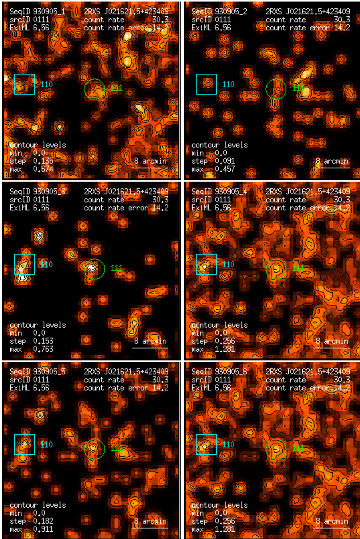
Figure 111: RASS 930905: detection 0111: band rate images, Gaussian filter: (1) PSPC channels 11 – 41, (2) 52 – 90, (3) 91 – 201, (4) 11 – 235, (5) 52 – 201, (6) 11 – 201. Broad band rates in counts/ks. Band rate contour levels in counts/ks/arcmin 2 .
