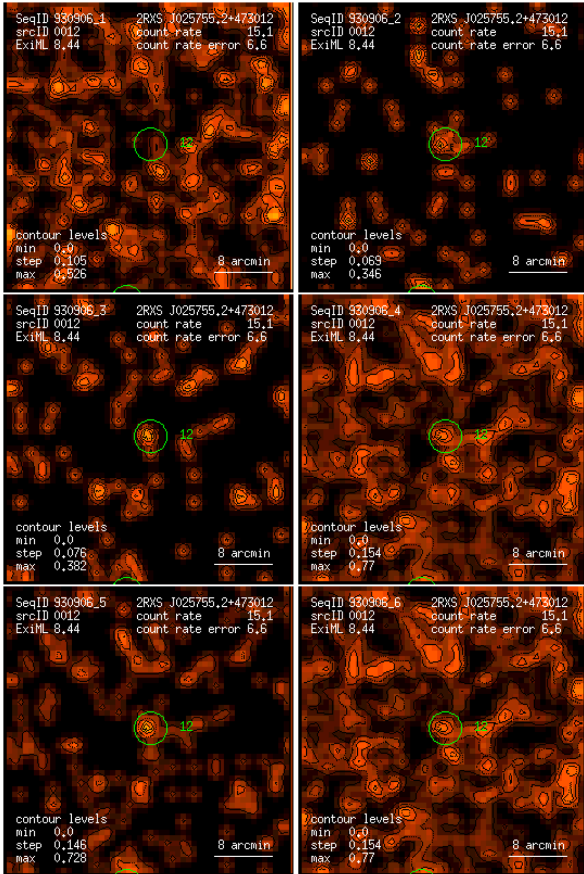
Figure 12: RASS 930906: detection 0012: band rate images, Gaussian filter: (1) PSPC channels 11 – 41, (2) 52 – 90, (3) 91 – 201, (4) 11 – 235, (5) 52 – 201, (6) 11 – 201. Broad band rates in counts/ks. Band rate contour levels in counts/ks/arcmin 2 .
