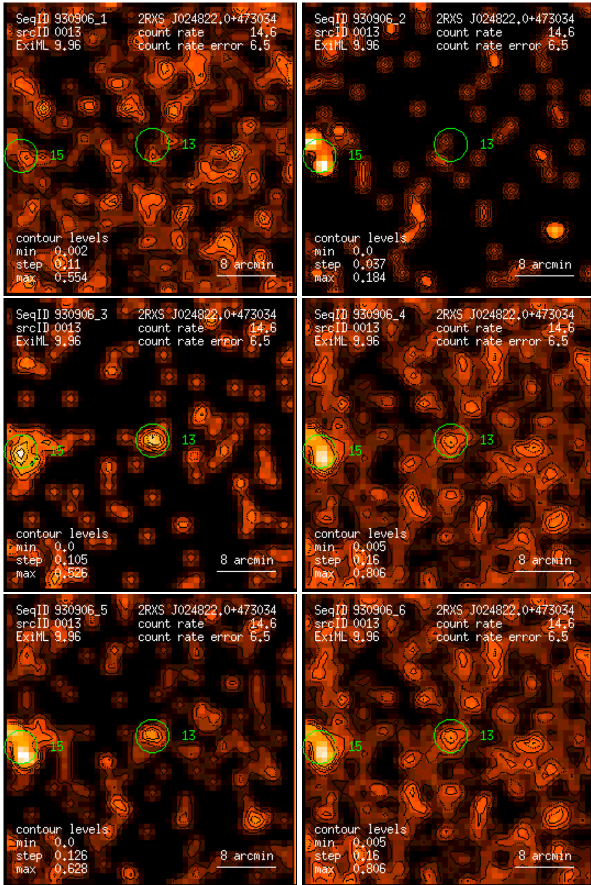
Figure 13: RASS 930906: detection 0013: band rate images, Gaussian filter: (1) PSPC channels 11 – 41, (2) 52 – 90, (3) 91 – 201, (4) 11 – 235, (5) 52 – 201, (6) 11 – 201. Broad band rates in counts/ks. Band rate contour levels in counts/ks/arcmin 2 .
