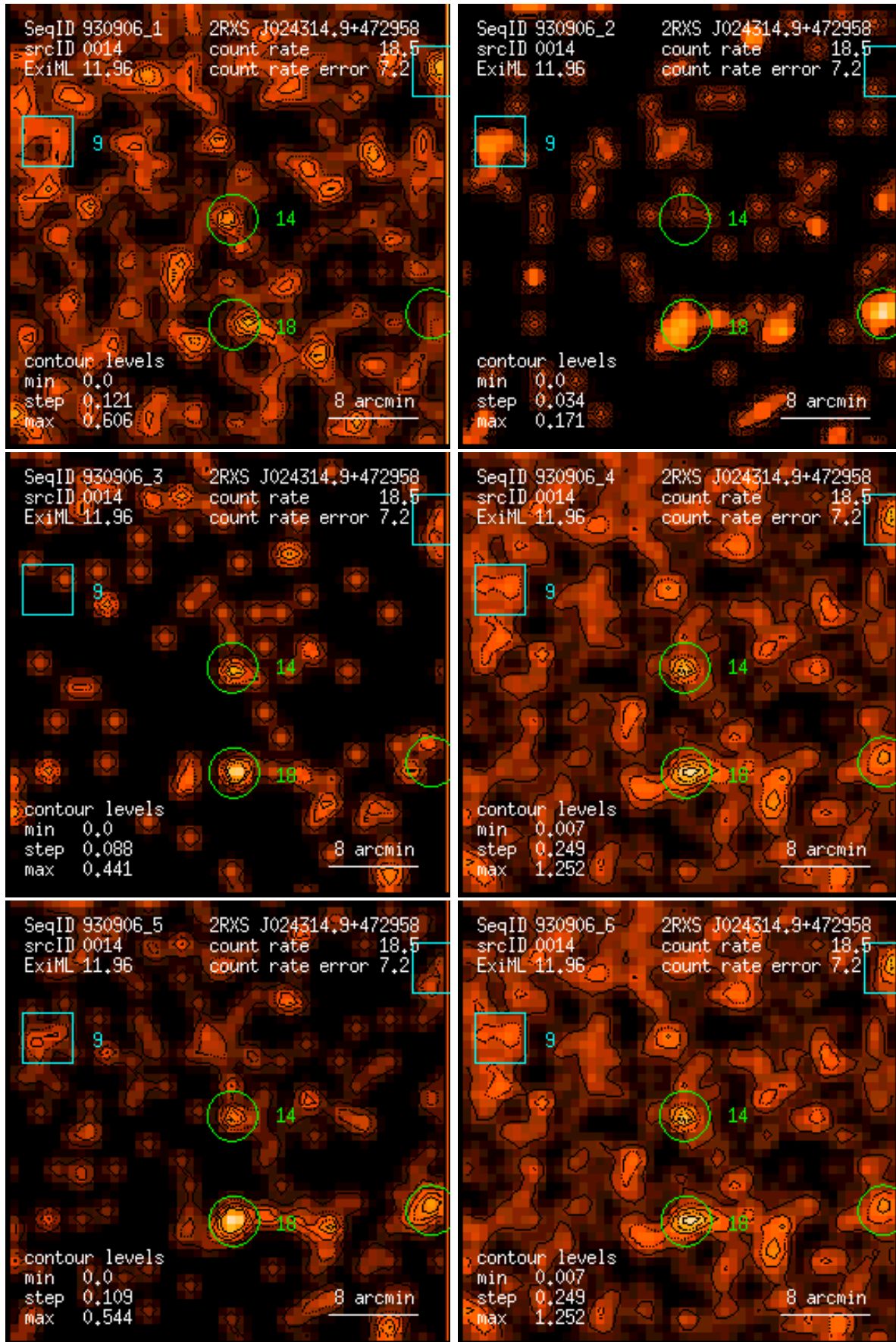
Figure 14: RASS 930906: detection 0014: band rate images, Gaussian filter: (1) PSPC channels 11 – 41, (2) 52 – 90, (3) 91 – 201, (4) 11 – 235, (5) 52 – 201, (6) 11 – 201. Broad band rates in counts/ks. Band rate contour levels in counts/ks/arcmin 2 .
