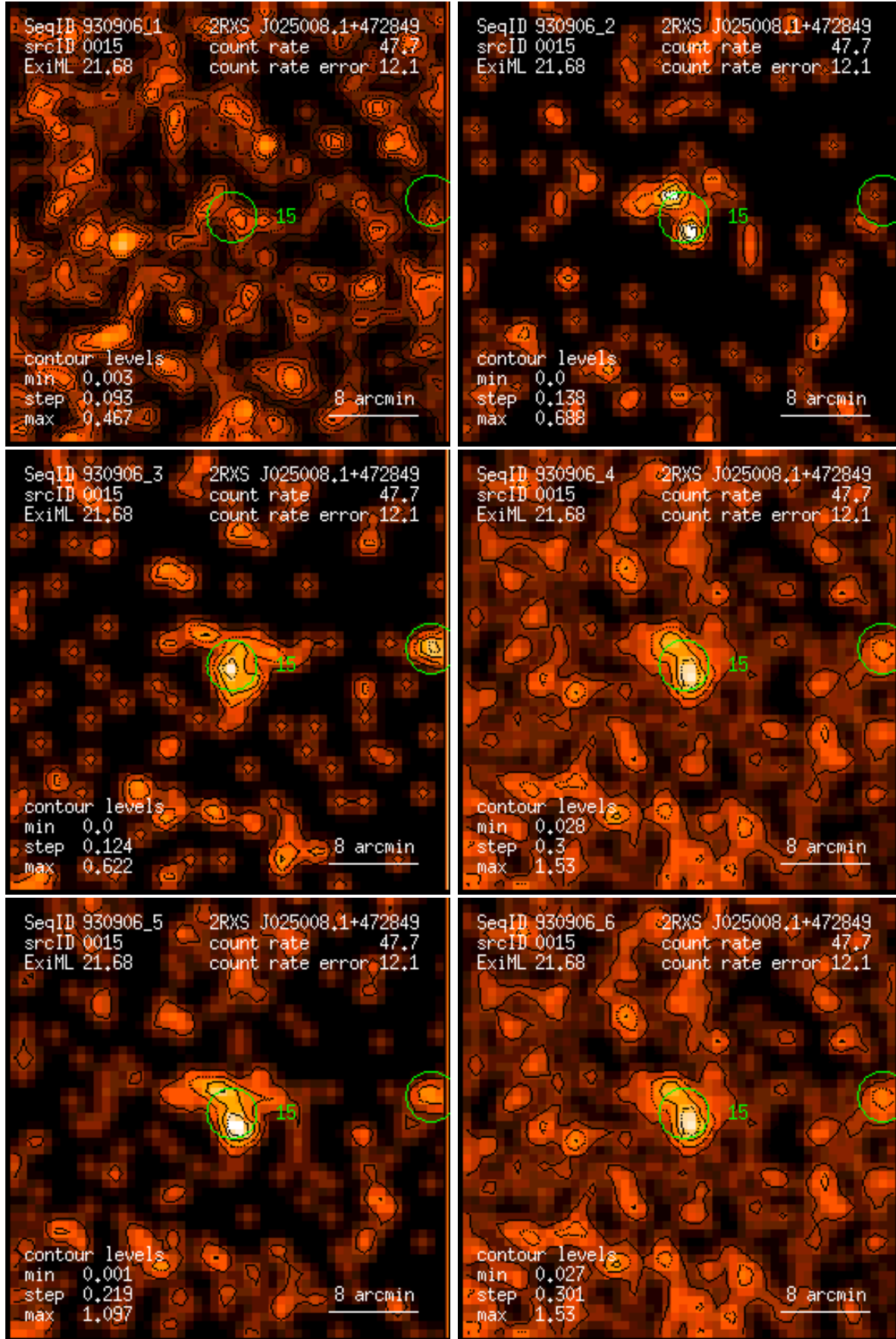
Figure 15: RASS 930906: detection 0015: band rate images, Gaussian filter: (1) PSPC channels 11 – 41, (2) 52 – 90, (3) 91 – 201, (4) 11 – 235, (5) 52 – 201, (6) 11 – 201. Broad band rates in counts/ks. Band rate contour levels in counts/ks/arcmin 2 .
