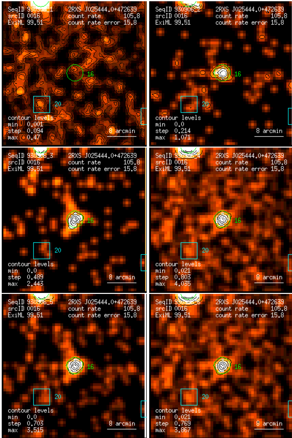
Figure 16: RASS 930906: detection 0016: band rate images, Gaussian filter: (1) PSPC channels 11 – 41, (2) 52 – 90, (3) 91 – 201, (4) 11 – 235, (5) 52 – 201, (6) 11 – 201. Broad band rates in counts/ks. Band rate contour levels in counts/ks/arcmin 2 .
