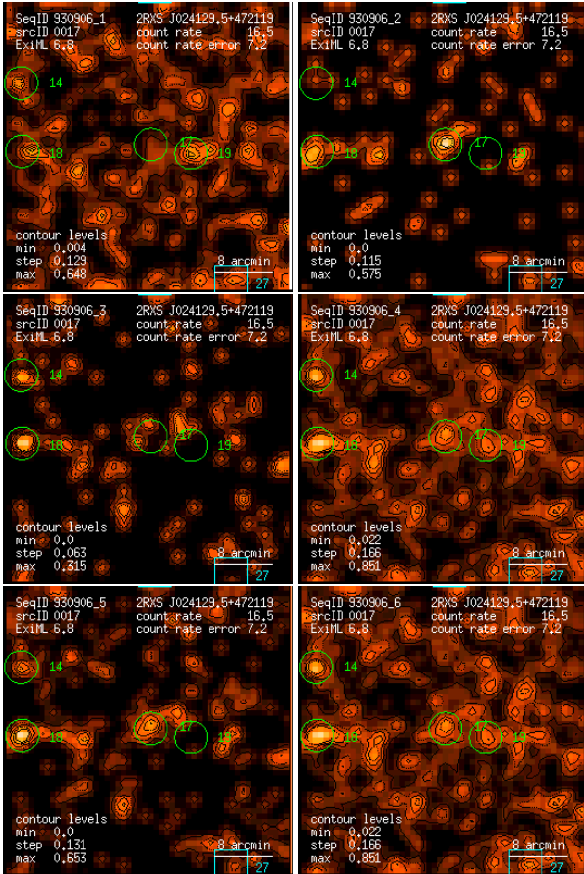
Figure 17: RASS 930906: detection 0017: band rate images, Gaussian filter: (1) PSPC channels 11 – 41, (2) 52 – 90, (3) 91 – 201, (4) 11 – 235, (5) 52 – 201, (6) 11 – 201. Broad band rates in counts/ks. Band rate contour levels in counts/ks/arcmin 2 .
