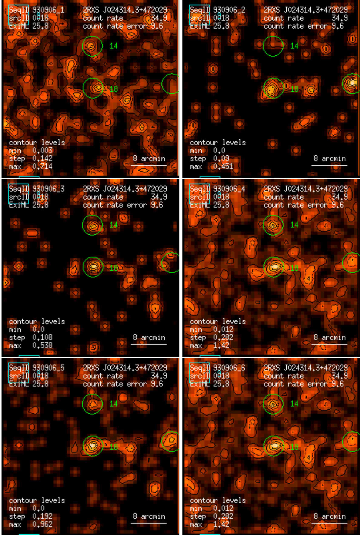
Figure 18: RASS 930906: detection 0018: band rate images, Gaussian filter: (1) PSPC channels 11 – 41, (2) 52 – 90, (3) 91 – 201, (4) 11 – 235, (5) 52 – 201, (6) 11 – 201. Broad band rates in counts/ks. Band rate contour levels in counts/ks/arcmin 2 .
