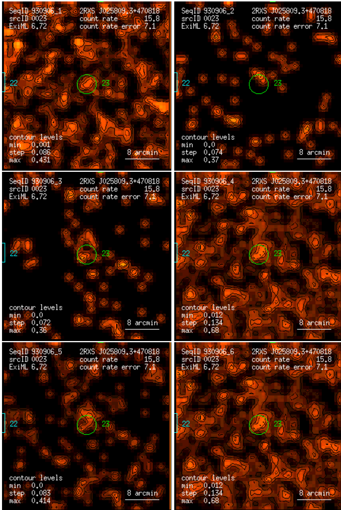
Figure 23: RASS 930906: detection 0023: band rate images, Gaussian filter: (1) PSPC channels 11 – 41, (2) 52 – 90, (3) 91 – 201, (4) 11 – 235, (5) 52 – 201, (6) 11 – 201. Broad band rates in counts/ks. Band rate contour levels in counts/ks/arcmin 2 .
