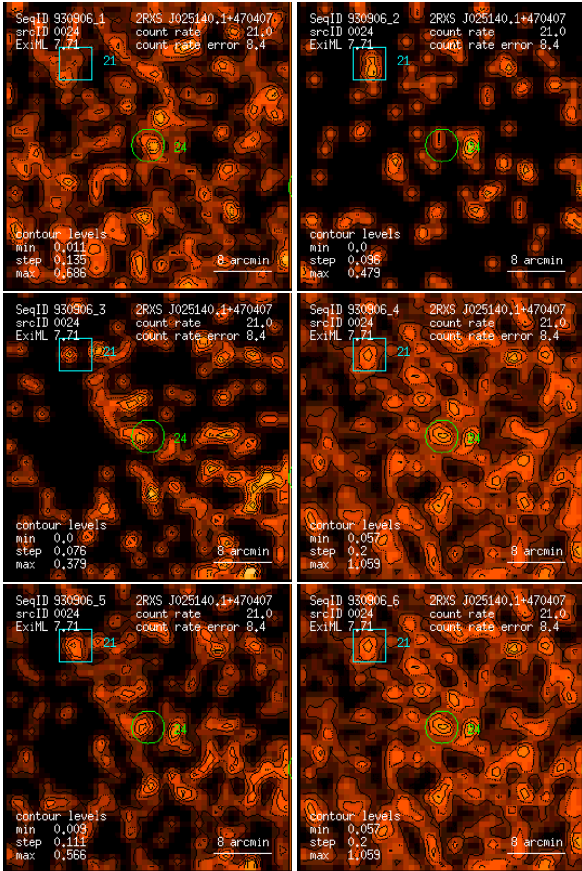
Figure 24: RASS 930906: detection 0024: band rate images, Gaussian filter: (1) PSPC channels 11 – 41, (2) 52 – 90, (3) 91 – 201, (4) 11 – 235, (5) 52 – 201, (6) 11 – 201. Broad band rates in counts/ks. Band rate contour levels in counts/ks/arcmin 2 .
