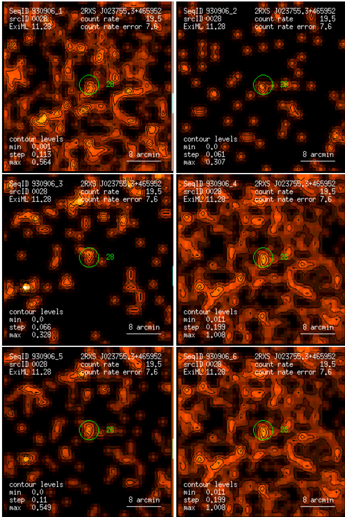
Figure 28: RASS 930906: detection 0028: band rate images, Gaussian filter: (1) PSPC channels 11 – 41, (2) 52 – 90, (3) 91 – 201, (4) 11 – 235, (5) 52 – 201, (6) 11 – 201. Broad band rates in counts/ks. Band rate contour levels in counts/ks/arcmin 2 .
