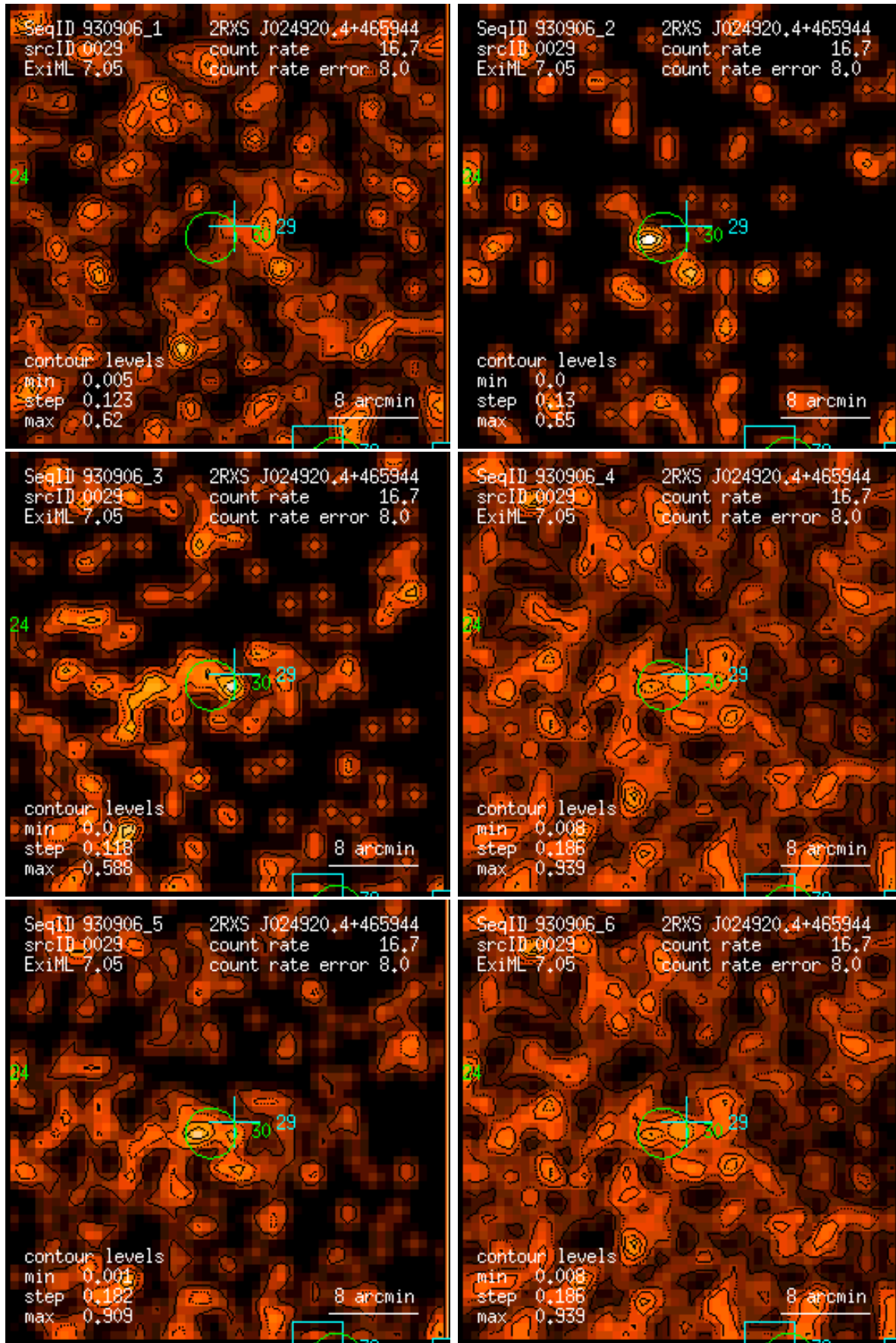
Figure 29: RASS 930906: detection 0029: band rate images, Gaussian filter: (1) PSPC channels 11 – 41, (2) 52 – 90, (3) 91 – 201, (4) 11 – 235, (5) 52 – 201, (6) 11 – 201. Broad band rates in counts/ks. Band rate contour levels in counts/ks/arcmin 2 .
