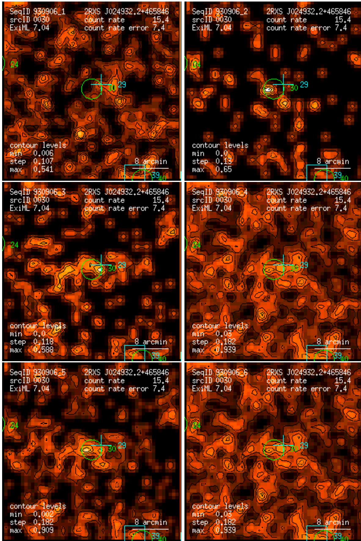
Figure 30: RASS 930906: detection 0030: band rate images, Gaussian filter: (1) PSPC channels 11 – 41, (2) 52 – 90, (3) 91 – 201, (4) 11 – 235, (5) 52 – 201, (6) 11 – 201. Broad band rates in counts/ks. Band rate contour levels in counts/ks/arcmin 2 .
