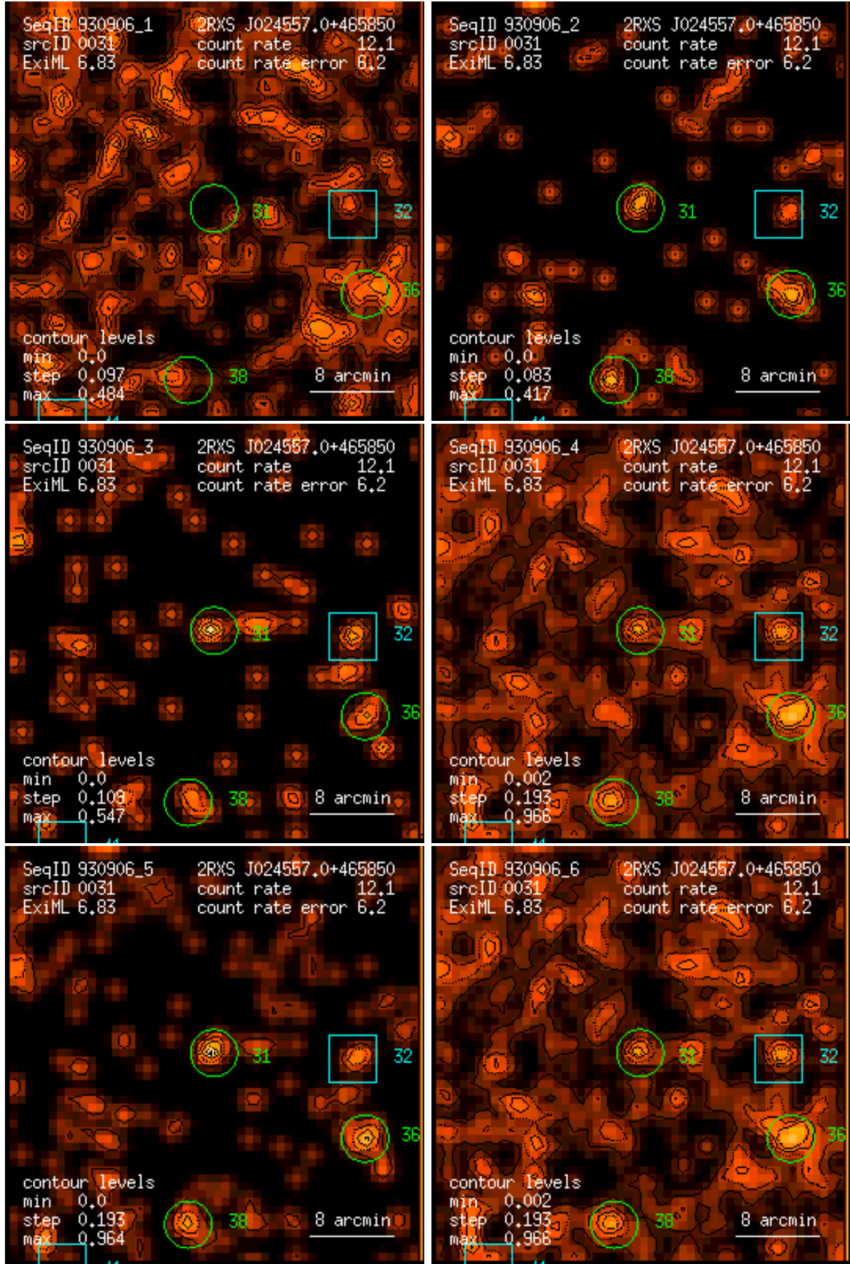
Figure 31: RASS 930906: detection 0031: band rate images, Gaussian filter: (1) PSPC channels 11 – 41, (2) 52 – 90, (3) 91 – 201, (4) 11 – 235, (5) 52 – 201, (6) 11 – 201. Broad band rates in counts/ks. Band rate contour levels in counts/ks/arcmin 2 .
