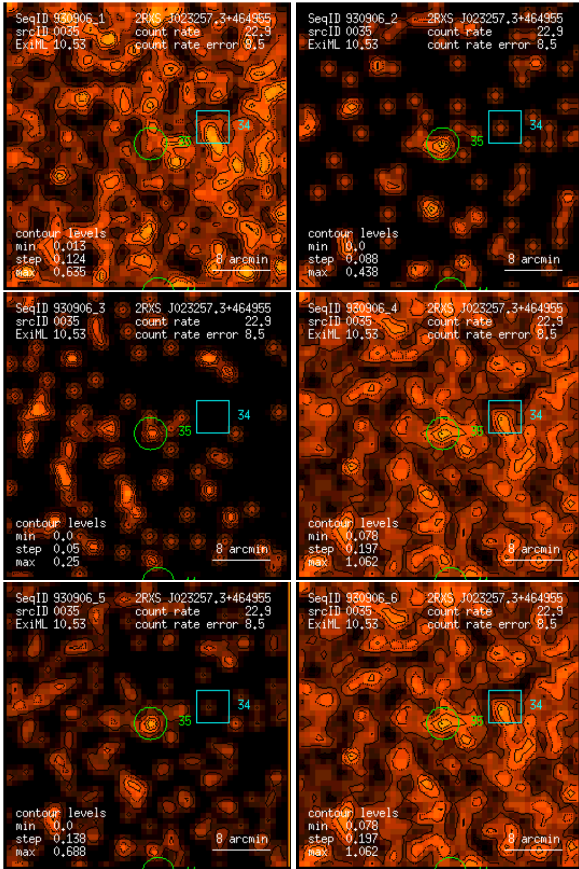
Figure 35: RASS 930906: detection 0035: band rate images, Gaussian filter: (1) PSPC channels 11 – 41, (2) 52 – 90, (3) 91 – 201, (4) 11 – 235, (5) 52 – 201, (6) 11 – 201. Broad band rates in counts/ks. Band rate contour levels in counts/ks/arcmin 2 .
