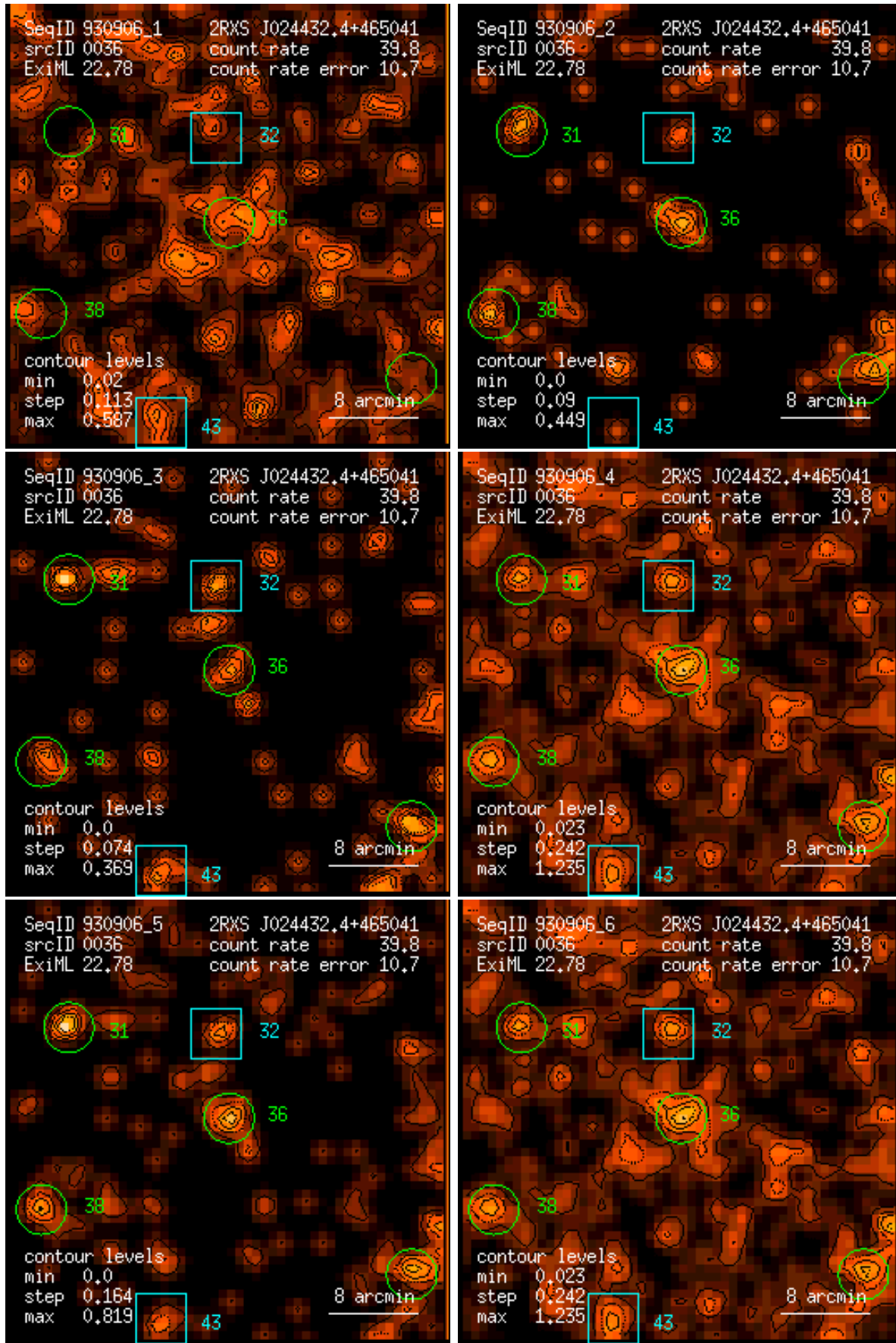
Figure 36: RASS 930906: detection 0036: band rate images, Gaussian filter: (1) PSPC channels 11 – 41, (2) 52 – 90, (3) 91 – 201, (4) 11 – 235, (5) 52 – 201, (6) 11 – 201. Broad band rates in counts/ks. Band rate contour levels in counts/ks/arcmin 2 .
