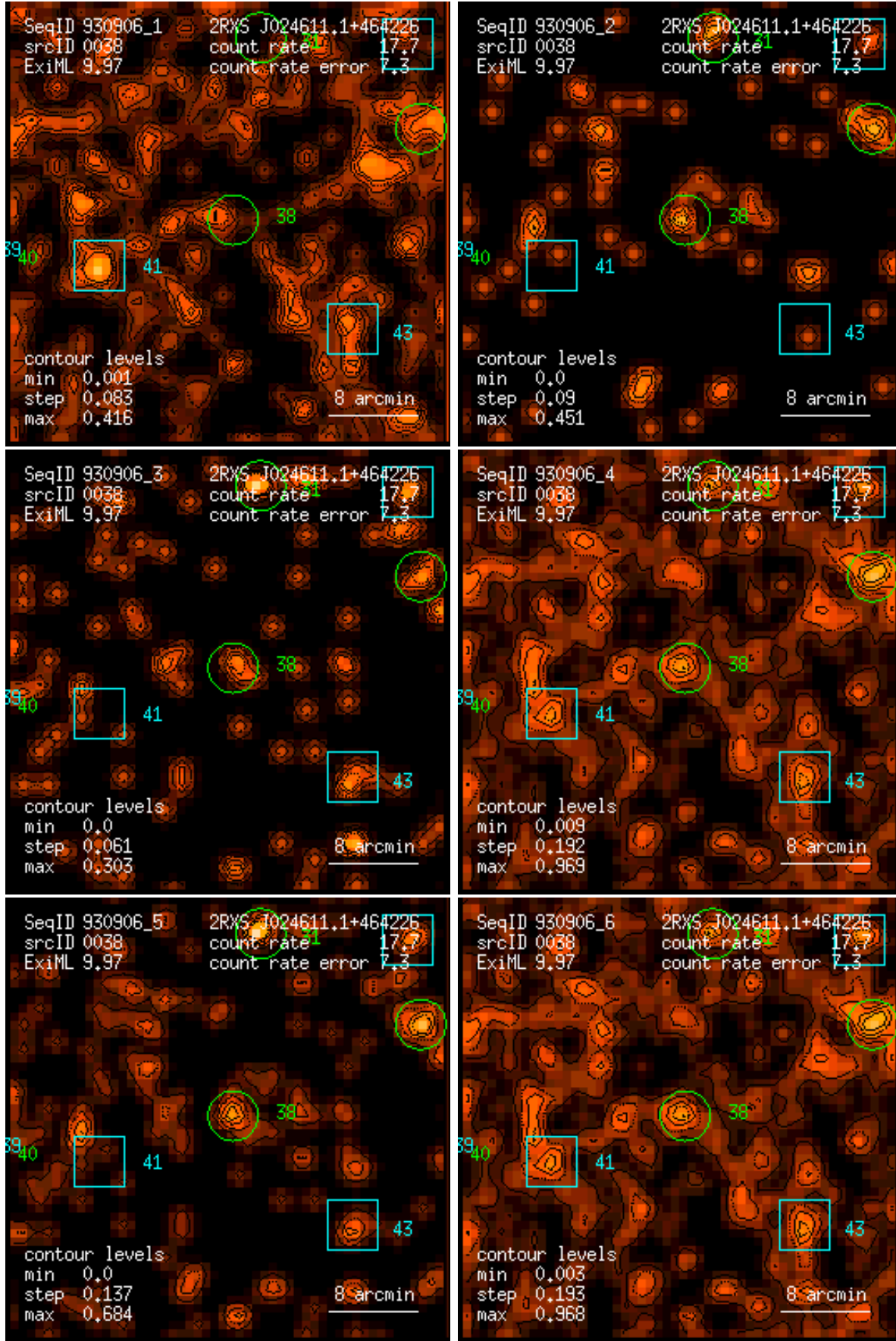
Figure 38: RASS 930906: detection 0038: band rate images, Gaussian filter: (1) PSPC channels 11 – 41, (2) 52 – 90, (3) 91 – 201, (4) 11 – 235, (5) 52 – 201, (6) 11 – 201. Broad band rates in counts/ks. Band rate contour levels in counts/ks/arcmin 2 .
