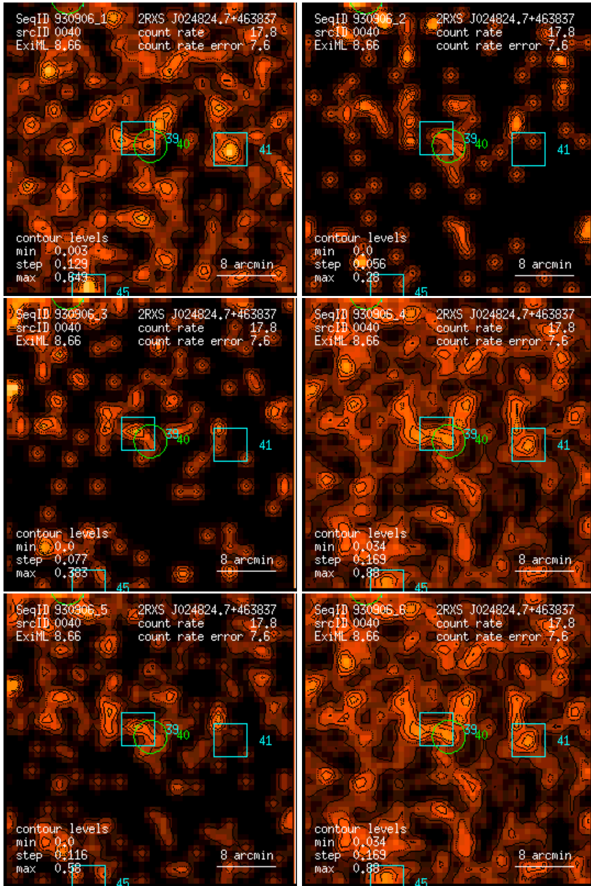
Figure 40: RASS 930906: detection 0040: band rate images, Gaussian filter: (1) PSPC channels 11 – 41, (2) 52 – 90, (3) 91 – 201, (4) 11 – 235, (5) 52 – 201, (6) 11 – 201. Broad band rates in counts/ks. Band rate contour levels in counts/ks/arcmin 2 .
