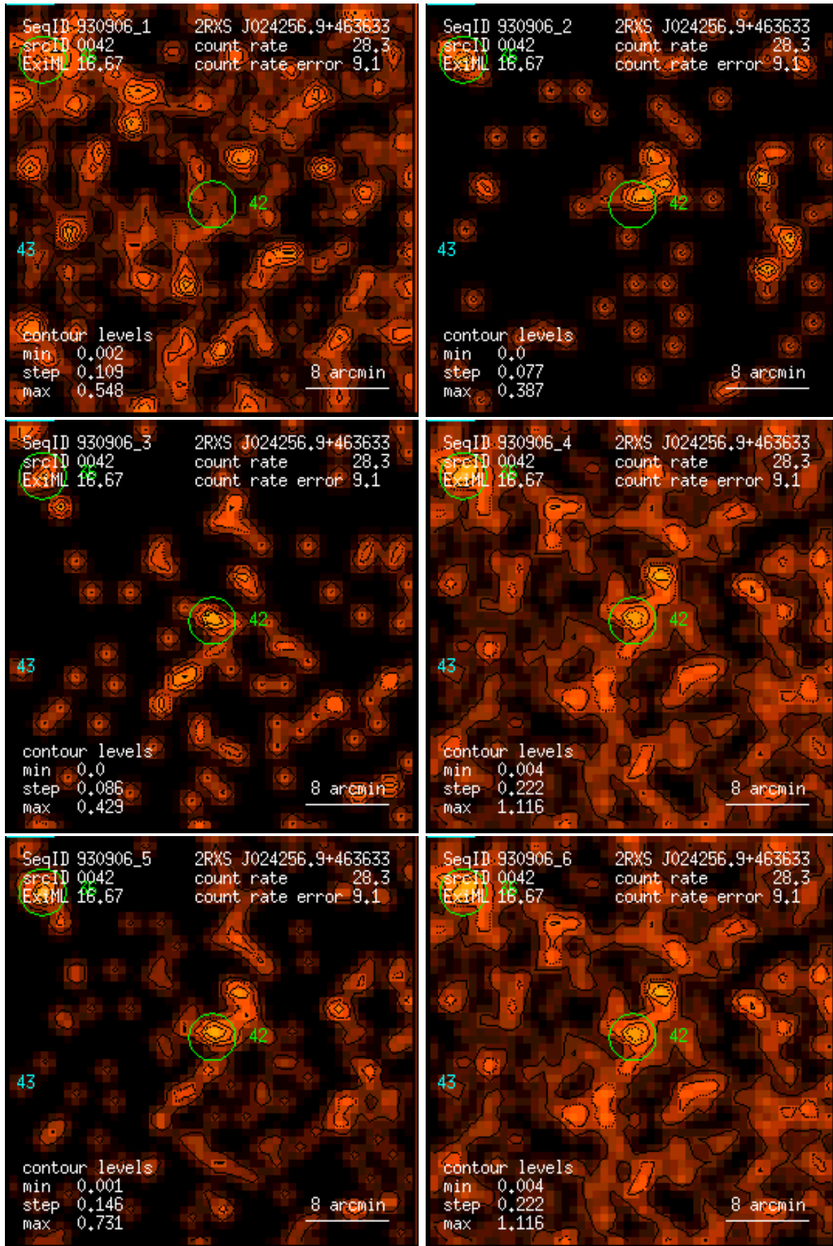
Figure 42: RASS 930906: detection 0042: band rate images, Gaussian filter: (1) PSPC channels 11 – 41, (2) 52 – 90, (3) 91 – 201, (4) 11 – 235, (5) 52 – 201, (6) 11 – 201. Broad band rates in counts/ks. Band rate contour levels in counts/ks/arcmin 2 .
