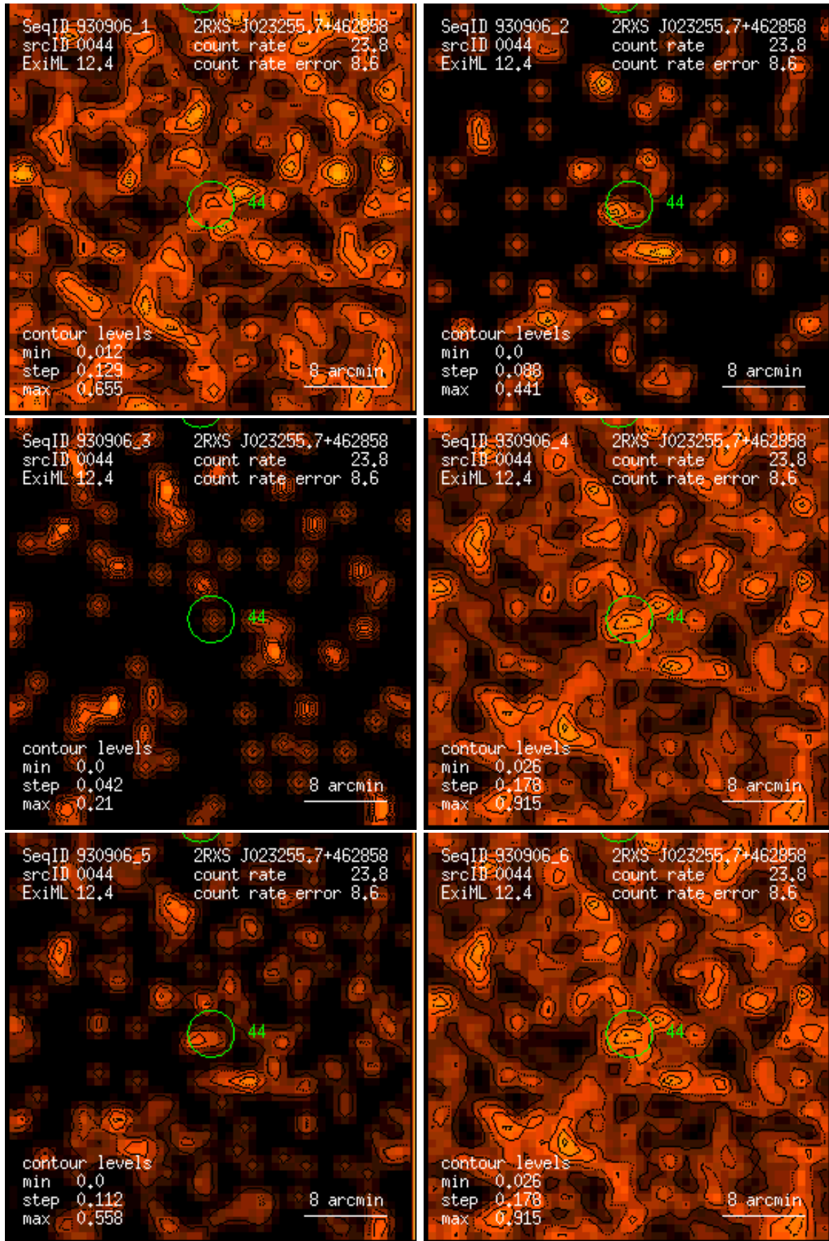
Figure 44: RASS 930906: detection 0044: band rate images, Gaussian filter: (1) PSPC channels 11 – 41, (2) 52 – 90, (3) 91 – 201, (4) 11 – 235, (5) 52 – 201, (6) 11 – 201. Broad band rates in counts/ks. Band rate contour levels in counts/ks/arcmin 2 .
