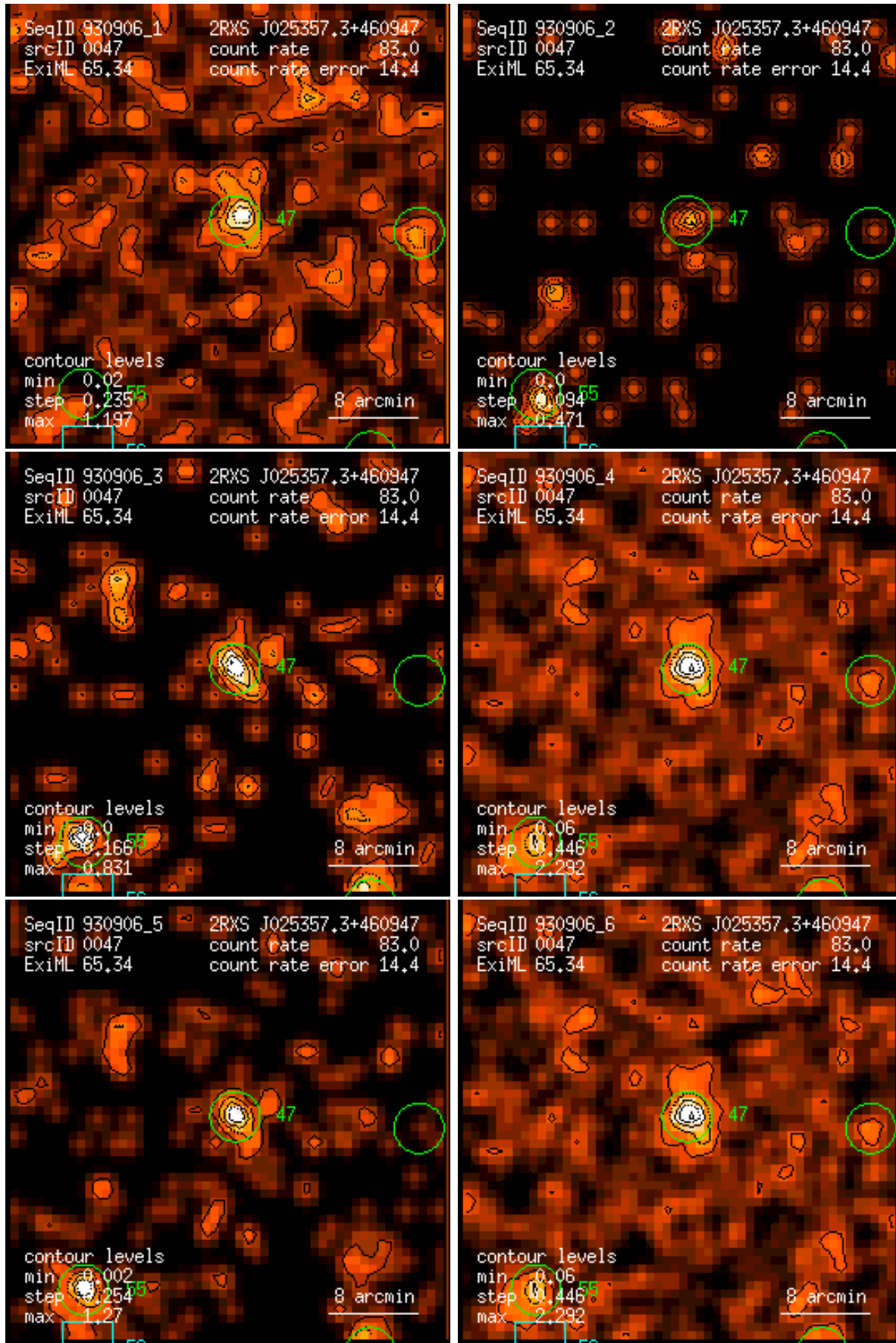
Figure 47: RASS 930906: detection 0047: band rate images, Gaussian filter: (1) PSPC channels 11 – 41, (2) 52 – 90, (3) 91 – 201, (4) 11 – 235, (5) 52 – 201, (6) 11 – 201. Broad band rates in counts/ks. Band rate contour levels in counts/ks/arcmin 2 .
