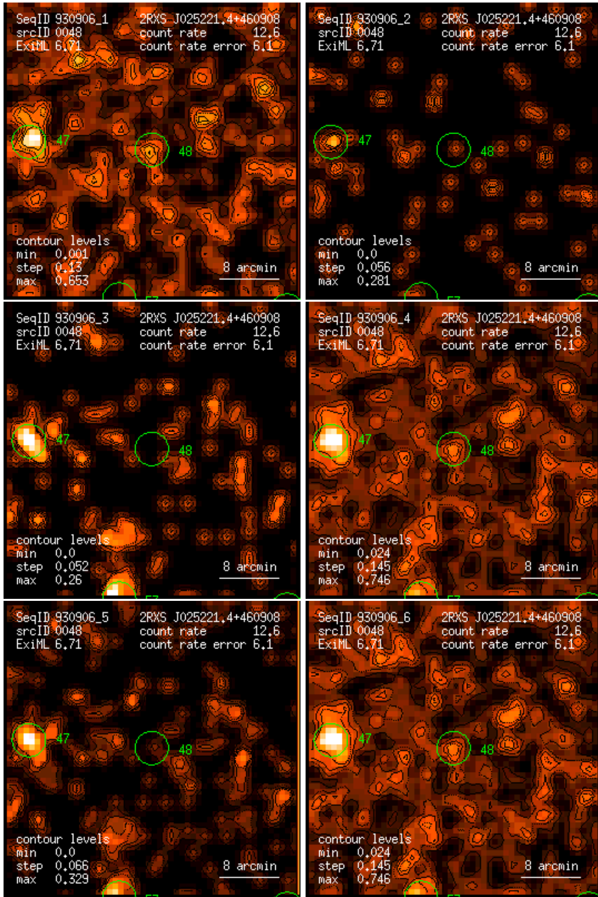
Figure 48: RASS 930906: detection 0048: band rate images, Gaussian filter: (1) PSPC channels 11 – 41, (2) 52 – 90, (3) 91 – 201, (4) 11 – 235, (5) 52 – 201, (6) 11 – 201. Broad band rates in counts/ks. Band rate contour levels in counts/ks/arcmin 2 .
