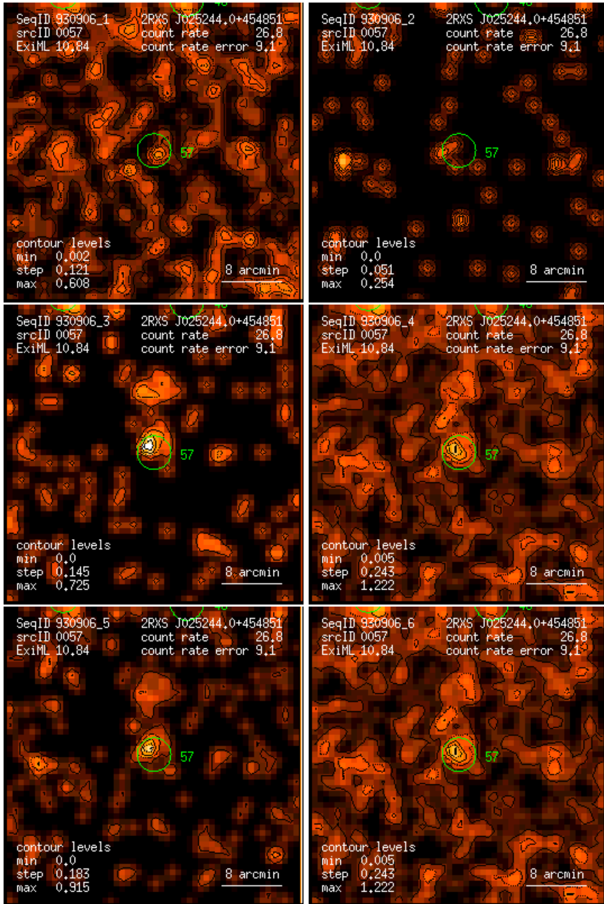
Figure 57: RASS 930906: detection 0057: band rate images, Gaussian filter: (1) PSPC channels 11 – 41, (2) 52 – 90, (3) 91 – 201, (4) 11 – 235, (5) 52 – 201, (6) 11 – 201. Broad band rates in counts/ks. Band rate contour levels in counts/ks/arcmin 2 .
