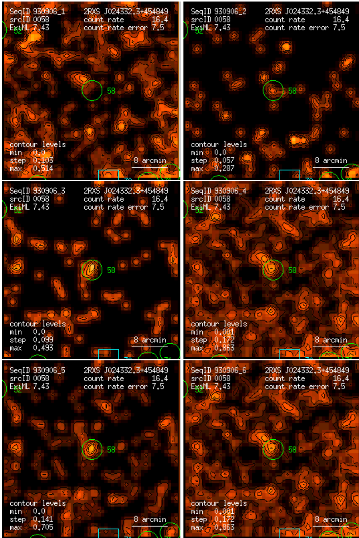
Figure 58: RASS 930906: detection 0058: band rate images, Gaussian filter: (1) PSPC channels 11 – 41, (2) 52 – 90, (3) 91 – 201, (4) 11 – 235, (5) 52 – 201, (6) 11 – 201. Broad band rates in counts/ks. Band rate contour levels in counts/ks/arcmin 2 .
