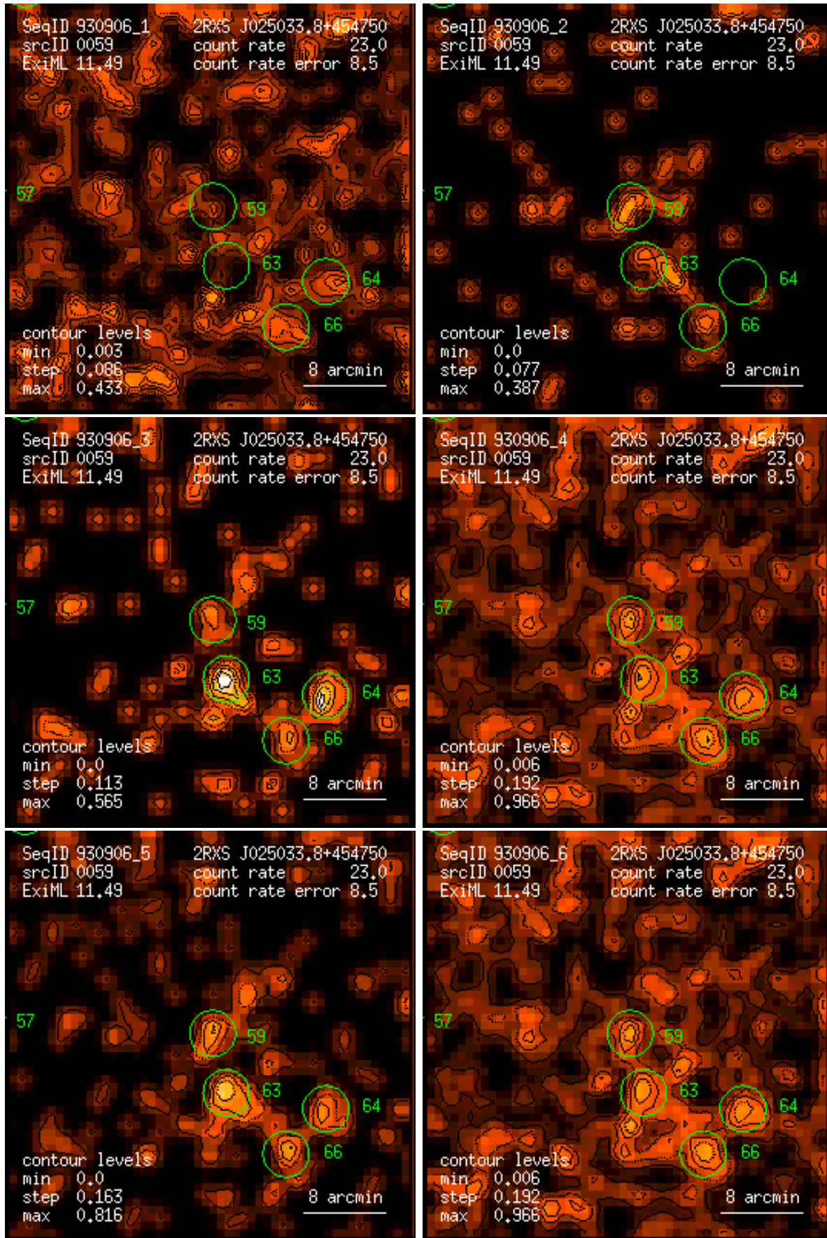
Figure 59: RASS 930906: detection 0059: band rate images, Gaussian filter: (1) PSPC channels 11 – 41, (2) 52 – 90, (3) 91 – 201, (4) 11 – 235, (5) 52 – 201, (6) 11 – 201. Broad band rates in counts/ks. Band rate contour levels in counts/ks/arcmin 2 .
