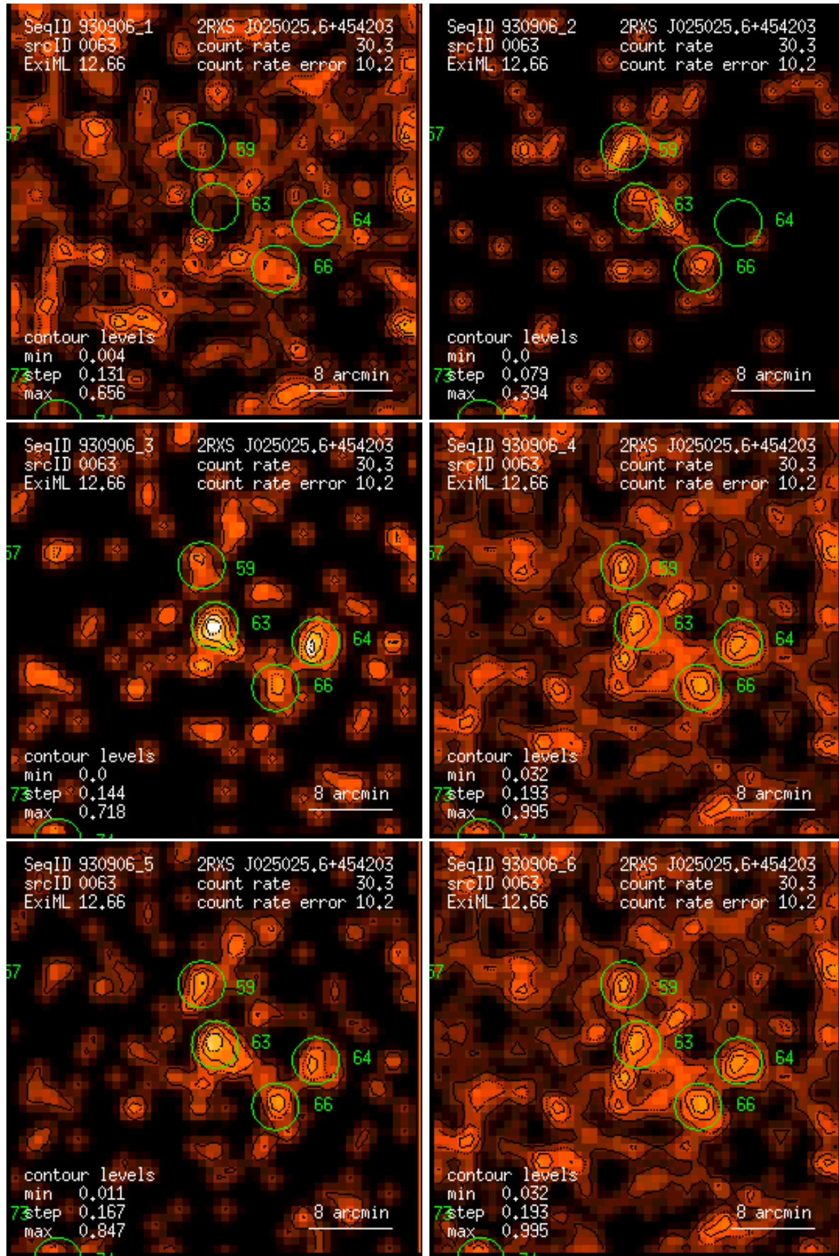
Figure 63: RASS 930906: detection 0063: band rate images, Gaussian filter: (1) PSPC channels 11 – 41, (2) 52 – 90, (3) 91 – 201, (4) 11 – 235, (5) 52 – 201, (6) 11 – 201. Broad band rates in counts/ks. Band rate contour levels in counts/ks/arcmin 2 .
