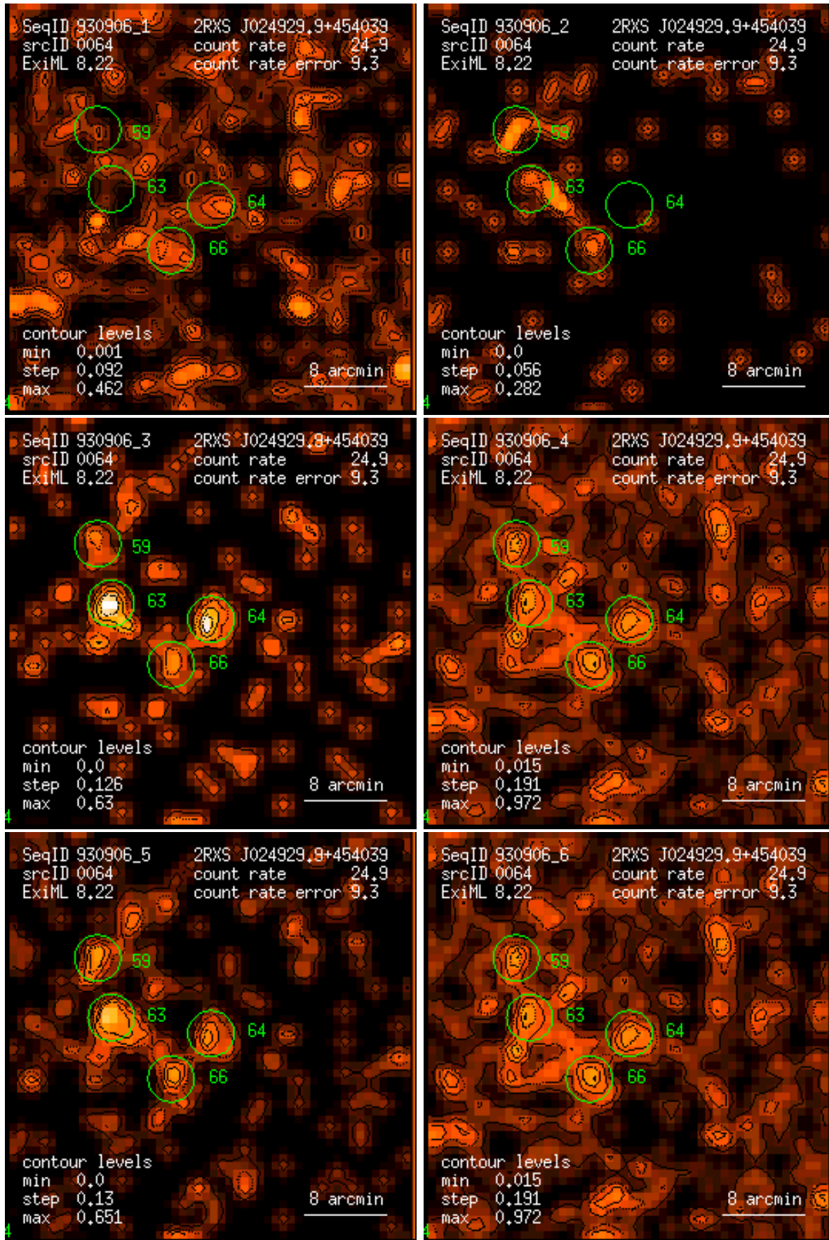
Figure 64: RASS 930906: detection 0064: band rate images, Gaussian filter: (1) PSPC channels 11 – 41, (2) 52 – 90, (3) 91 – 201, (4) 11 – 235, (5) 52 – 201, (6) 11 – 201. Broad band rates in counts/ks. Band rate contour levels in counts/ks/arcmin 2 .
