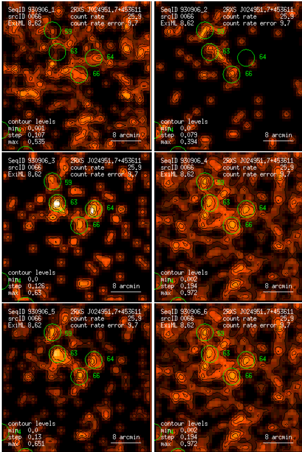
Figure 66: RASS 930906: detection 0066: band rate images, Gaussian filter: (1) PSPC channels 11 – 41, (2) 52 – 90, (3) 91 – 201, (4) 11 – 235, (5) 52 – 201, (6) 11 – 201. Broad band rates in counts/ks. Band rate contour levels in counts/ks/arcmin 2 .
